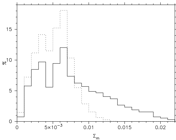
Fig. 5. Distribution of \Sigma_m , which is a measure of the fit quality averaged over the line profile and expressed in continuum units – see Eq. (1), for 3600 fits without macroturbulence (full line) and with macroturbulence (either A_{ISO} , A_R , or A_T whichever gave the lowest \Sigma_m , dotted line).
