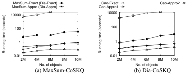
Figure 7: Scalability Test
