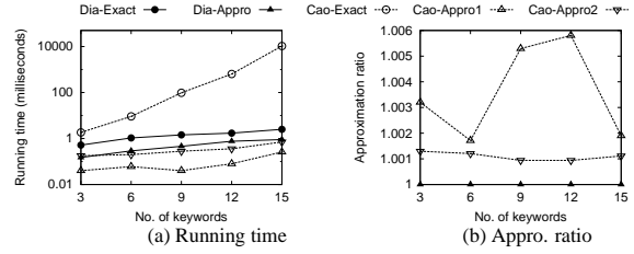
Figure 8: Effect of |\mathcal{O}_q| (GN, Dia-CoSKQ)
