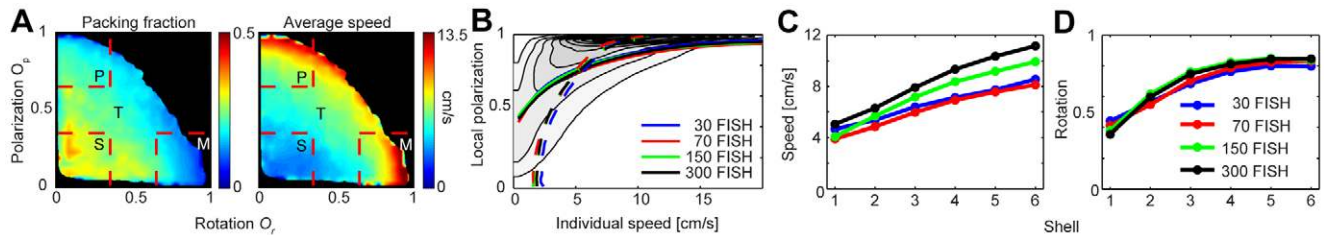
Figure 7. Structural properties. (A) Density plots of packing fraction and average individual speed (averaged per frame) as functions of rotation O_r and polarization O_p for 150 fish. (B) The plot illustrates the correlation between individual speed and local polarization estimated in two ways from the underlying density maps (the example shown in the background is for 150 fish). The stapled curves are produced by averaging across individual speeds for each value of the order parameter; the solid curves from averaging across the order parameter values for each individual speed. The local polarization of an individual fish is defined as the polarization O_p restricted to the area inside a circle with radius 15.6 cm (approximately 3 body lengths) centered at the individual fish. (C) Average individual speed at different radial positions in the milling state. (D) Average rotational order parameter at the same positions. The radial division of the milling state in (C) and (D) is constructed by centering six shells outside each other, where the outermost shell has a radius defined by the distance from the group's center of mass to the median distance of the five most peripheral fish (see illustration in Fig. S11). The width of each shell is the radius of the outer shell divided by six. The averages are calculated for each shell, where the outer shell even includes peripheral fish. doi:10.1371/journal.pcbi.1002915.g007
