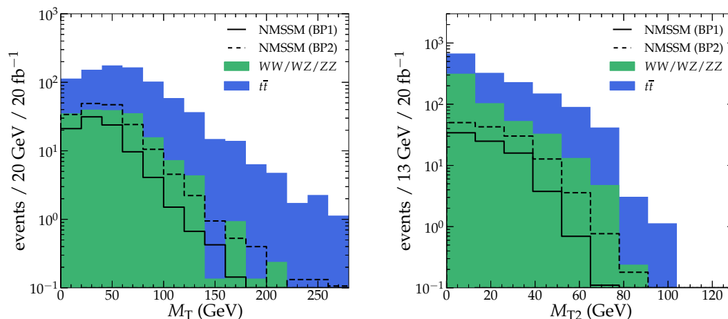
Figure 10. Distributions of (left panel) transverse mass for one lepton + missing energy and (right panel) and the M_{T2} for an opposite-sign lepton pair and missing energy. Background distributions are normalized to match the signal distributions. The basic event selection cuts are applied for both signals and backgrounds.
