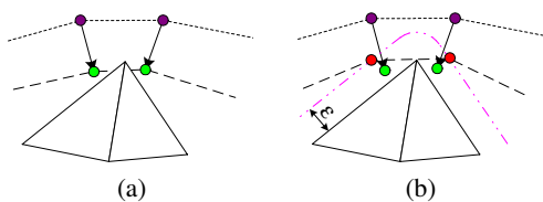
Figure 14: (a) Without offsetting the vertices, penetration artifacts may occur during collision detection. (b) Introducing an \epsilon -offset solves the problem.
