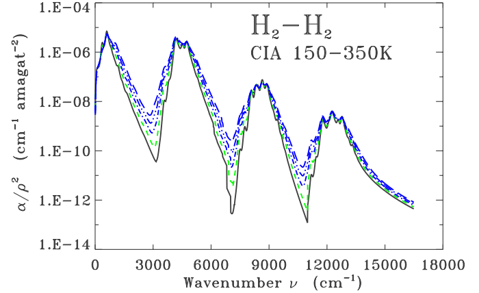
Fig. 1. CIA spectra of hydrogen pairs computed at temperatures 150 K (lowest solid line), 200 K, 250 K, 300 K and 350 K (uppermost line).
