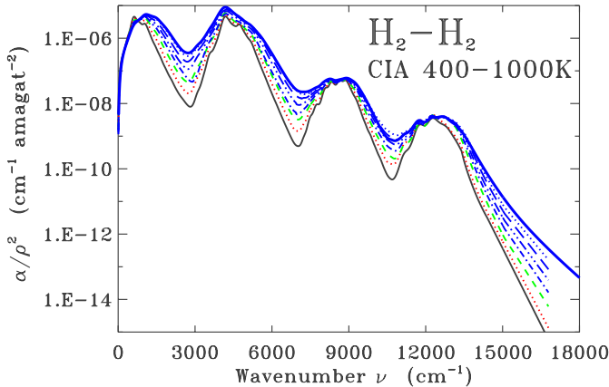
Fig. 2. The CIA spectra of hydrogen pairs computed at temperatures from 400 to 1000 K. Spectra are given at 400 K (lowest lying solid line), 500 K, 600 K, 700 K, 800 K, 900 K and 1000 K (upper dotted line ending at 17000 cm -1 ). For comparison, the results obtained by Borysow et al. (2001) at 1000 K are also shown (thick, uppermost, solid line).
