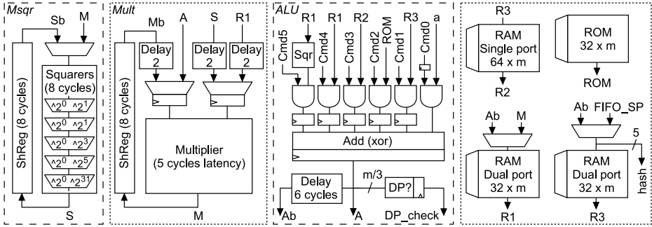
Fig. 2. Medium processor, Point Update unit (squarers for m = 163 )
