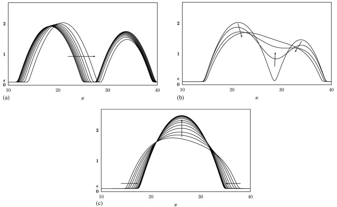
Fig. 11. Details of the collision and merging process: (a) two near-equilibrium droplet evolving toward collision, (b) the formation of the collided “two-drop complex” and its rapid convexification, (c) symmetrization and contraction to yield a single merged near-equilibrium droplet.
