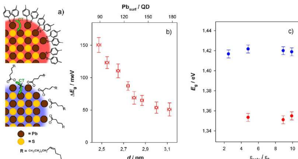
Figure 3. (a) Drawings illustrating the relaxation of exciton confinement in PbS/ArS QDs (red nuance), due to the ArS-to-QD CT interactions (green arrow); in PbS/OI QDs, the exciton is instead confined on the inorganic core (blue nuance), resulting from the lack of interfacial CT interactions as for lead(II)–carboxylate complexes. (b) Plot of the optical band gap reduction, \Delta E_g , as a function of QD diameter, d , and of the number of excess Pb atoms on the QD surface. (c) Plot of the optical band gap of PbS/OI QDs (blue circles) and PbS/ArS QDs (red circles) in chlorinated solvents characterized by increasing dielectric constant: tetrachloroethylene, chloroform, DCM, and DCB, respectively; PbS/ArS QDs are poorly soluble in tetrachloroethylene. Symbols and error bars represent the average value and one standard deviation, respectively, calculated from at least three measurements.
