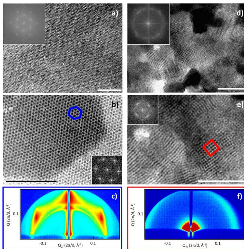
Figure 4. (a,b,d,e) TEM images at different magnification of 2.8 nm PbS QD self-assemblies capped with OL (a,b) and ArS (d,e) molecules. Scale bar is 100 nm (a,d) or 50 nm (b,e). Polygons are drawn to emphasize the different packing motifs adopted by PbS/OL QDs and PbS/ArS QDs. Insets show fast Fourier transform of the corresponding images. (c,f) GISAXS patterns of 2.8 nm PbS QD self-assemblies capped with OL (c) and ArS (f) molecules.
