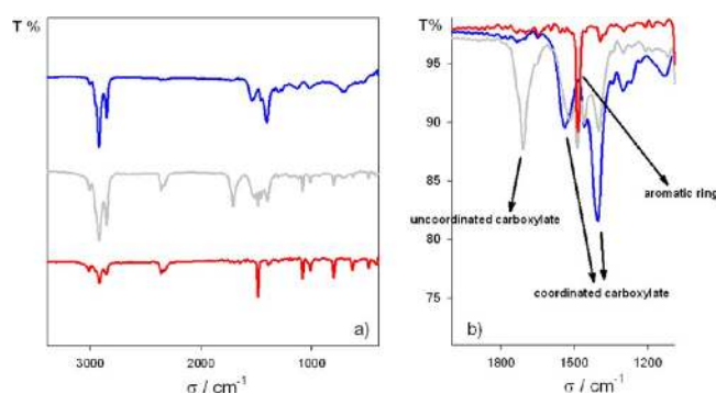
Figure 1. (a,b) FTIR spectra of thin films of PbS/OI QDs (blue line), PbS/OI QDs upon addition of \text{ArS}^-/\text{TEA}\cdot\text{H}^+ (gray line), and purified PbS/ArS QDs (red line). (b) Details of the FTIR spectra showing the stretching peaks at 1400 and 1540 \text{cm}^{-1} of QD-coordinated carboxylate moieties in PbS/OI QDs (blue line), at 1700 \text{cm}^{-1} of uncoordinated carboxylate moieties upon \text{ArS}^-/\text{TEA}\cdot\text{H}^+ addition (gray line), and at 1490 \text{cm}^{-1} of the aromatic ring in purified PbS/ArS QDs (red line). The features around 2350 \text{cm}^{-1} correspond to the asymmetric stretching of carbon dioxide in air.
