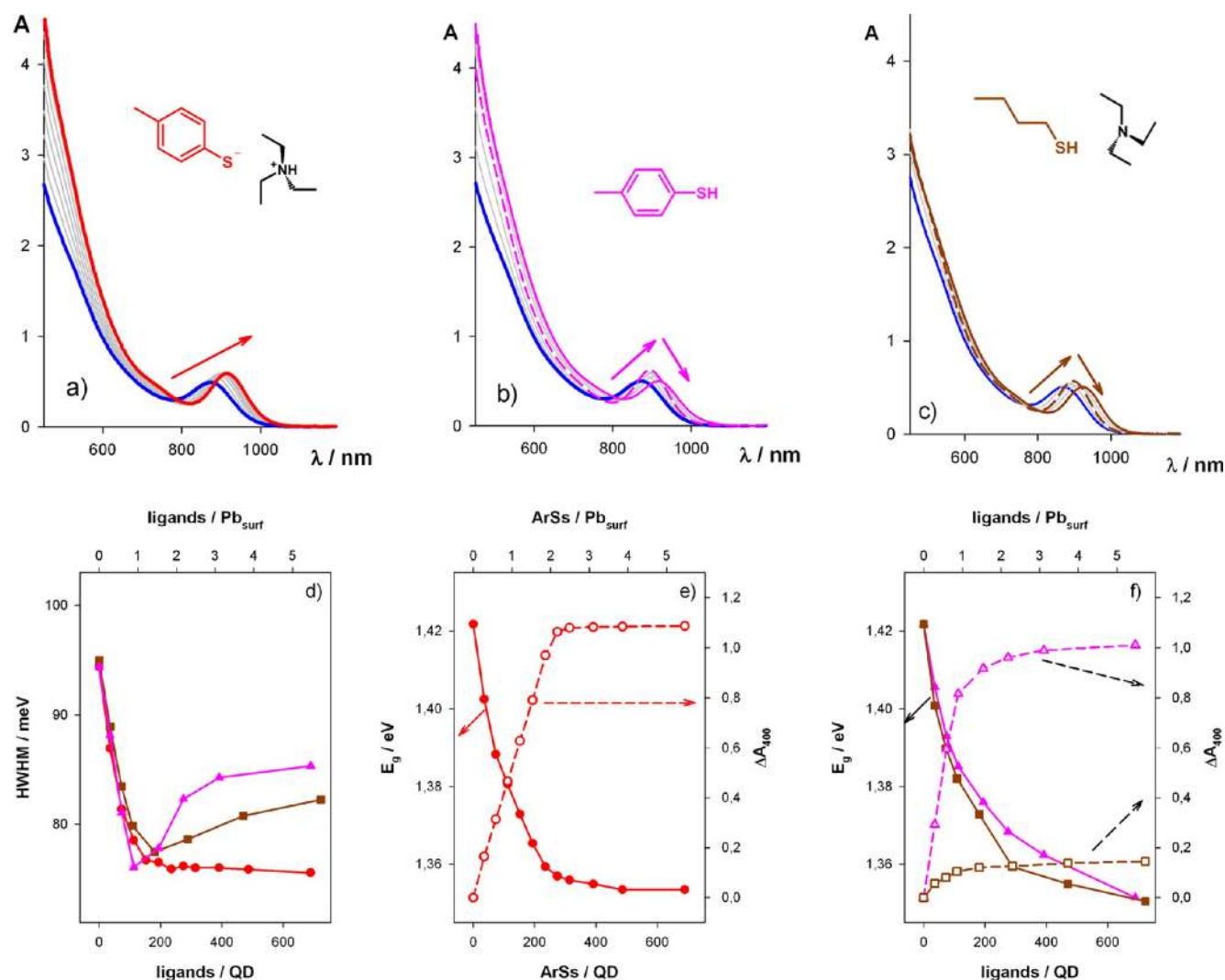
Figure 2. (a,b,c) Optical absorption spectra of 9.8 \mu M air-equilibrated DCM solution of PbS/OI QDs (blue spectrum) upon addition of (a) \text{ArS}^-/\text{TEA}\cdot\text{H}^+ (red spectrum), (b) \text{ArS}\cdot\text{H}^+ (pink spectrum), and (c) \text{AlSH}/\text{TEA} (brown spectrum) up to 700 equiv. (d) Plot of the narrowing of the first excitonic peak of PbS QDs upon titration with \text{ArS}^-/\text{TEA}\cdot\text{H}^+ (red circles), \text{ArS}\cdot\text{H}^+ (pink triangles), and \text{AlSH}/\text{TEA} (brown squares). (e) Plots of the reduction of the optical band gap (full red circles) and the absorbance increase at 400 nm (empty red circles) upon addition of \text{ArS}^-/\text{TEA}\cdot\text{H}^+ to a 1.8 mM solution of PbS/OI QDs in DCM, showing that spectral changes reach a plateau when two \text{ArS}^- ligands per excess Pb atom on the QD surface are added. 38,42 (f) Plots of the reduction of the optical band gap (full symbols) and the absorbance increase at 400 nm (empty symbols) upon addition of \text{ArS}\cdot\text{H}^+ (pink triangles) and \text{AlSH}/\text{TEA} (brown squares) to a 1.8 mM solution of PbS/OI QDs in DCM.
