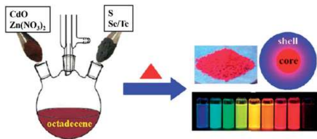
Fig. 12 Schematic illustration for the synthesis of cadmium chalcogenide core/shell NCs through non-injection methods (reproduced with permission from ref. 32, copyright 2012, American Chemical Society).
