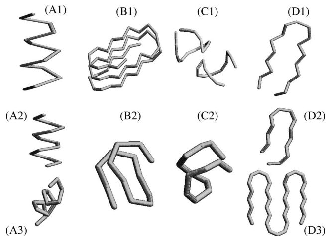
FIG. 5. Building blocks of biomolecules and ground-state structures associated with the marginally compact phase of a short tube. The top row shows some of the building blocks of biomolecules, while the second row depicts the corresponding structures obtained for a tube in the twilight zone. (A1) is an \alpha helix of a naturally occurring protein, while (A2) and (A3) are the helices obtained in our calculations. (A2) has a regular contact map whereas (A3) is a distorted helix in which the distance between successive atoms along the helical axis is not constant, but has period 2. (B1) is a helix of strands in the alkaline protease of Pseudomonas aeruginosa , whereas (B2) shows the corresponding structure obtained in our computer simulations. (C1) shows the “kissing hairpins” of RNA and (C2) the corresponding conformation obtained in our simulations. Finally (D1) and (D2) are two instances of quasiplanar hairpins. The first structure is from the same protein as before (the alkaline protease of Pseudomonas aeruginosa ) while the second is a typical conformation found in our simulations. The sheetlike structure (D3) is obtained for a longer tube. The tube thickness increases from left to right while the range of interactions is held fixed. For more details, see Banavar, Flammini, Marenduzzo, Maritan, and Trovato (2003).
