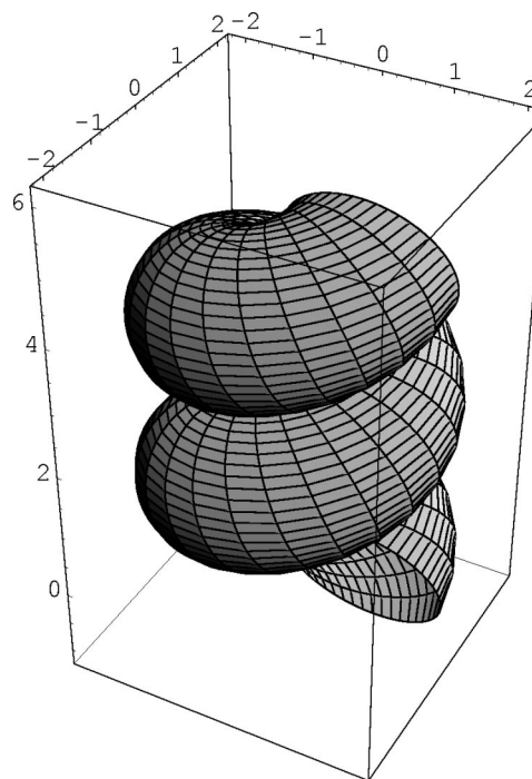
FIG. 2. Space-filling helix. The geometry of this helix nicely illustrates the idea behind the three-body potential. Consider a tube in a compact helical conformation. The smallest value that the local radius of curvature of the helix can adopt equals the tube thickness. Note that if the local radius of curvature were any smaller than the tube thickness, the tube would self-intersect and such configurations are not allowed. Physically, a space-filling helix is obtained when successive turns of the tube lie on top of each other. This translates into the observation that the nonlocal radius associated with three points, of which two are close together and the third is alongside them in a neighboring turn, is also equal to the tube thickness. Again, a radius smaller than this value would lead to an intersection and is forbidden. The pitch-to-radius ratio of this helix is within 3% of the corresponding value for \alpha helices in globular proteins.
