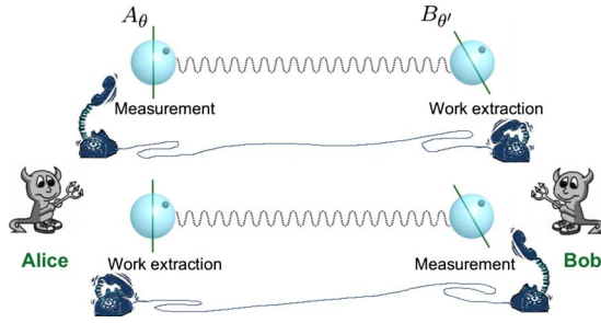
FIG. 13. (Color online) Schematic of the protocol to extract work from correlated pairs. Two pairs represent an ensemble for which Alice and Bob use A_\theta and B_{\theta'} for their measurement and work extraction. For a half of this ensemble, Alice measures her state with A_\theta and Bob extracts work from his side along the direction of \theta' , according to Alice's measurement results. For the other half, they exchange their roles.
