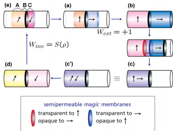
FIG. 8. (Color online) Thermodynamic cycle given by Peres to show that distinguishing nonorthogonal quantum states leads to a violation of the second law. The arrows indicate the directions of spin in the Bloch sphere. The use of hypothetical semipermeable membranes, which distinguish nonorthogonal states |\uparrow\rangle and |\rightarrow\rangle perfectly, in the step from (b) to (c) is the key to violate the second law. Adapted from Fig. 9.2 in Peres, 1993.
