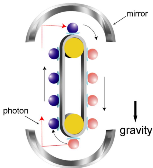
FIG. 9. (Color online) Bondi's thought experiment for a perpetual mobile. Excited atoms (on the right side and at the bottom of the belt) emit a photon at the bottom of the belt to lower its energy level. The emitted photon is reflected by the curved mirrors placed so that it will be absorbed by an atom in the lower energy level at the top of the belt.
