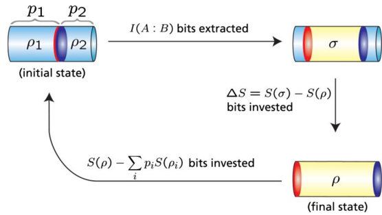
FIG. 11. (Color online) The thermodynamic cycle, which we use to discuss the second law. The cycle proceeds from the initial state to the final state \rho via the post-work-extraction state \sigma , and returns to the initial state with a reversible process.
