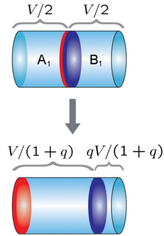
FIG. 6. (Color online) Possible configuration to confirm the continuity of the extractable work. The left- (right-) hand side of a chamber is filled with an A_1 ( B_1 ) gas. Two membranes that distinguish A_1 and A_2 are used to extract work. The membrane on the left lets the A_1 gas pass through it freely, but reflects the A_2 gas completely. The other membrane works in the opposite manner. Since the B_1 gas changes its state into A_1 with probability q when measured by the membrane, the right membrane does not reach the right end of the chamber by a (quasi-)isothermal expansion.
