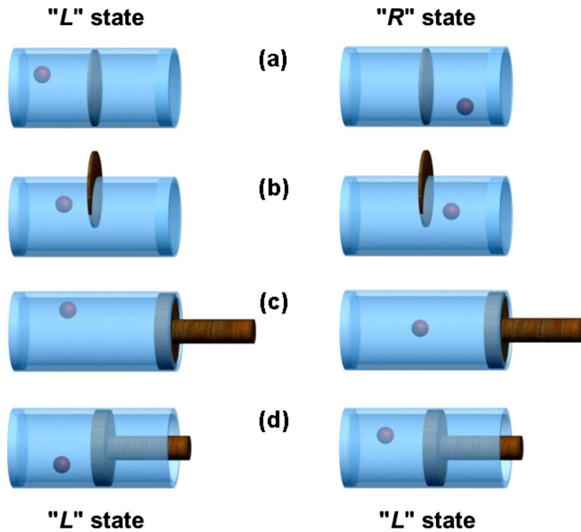
FIG. 3. (Color online) Thermodynamic process to erase information. Binary information is stored in a vessel as the position of the molecule, either L or R . A common procedure for both initial states, i.e., removing the partition and halving the whole volume by an isothermal compression towards the standard state L , completes the erasure. Adapted from Fig. 3 in Plenio and Vitelli, 2001 .
