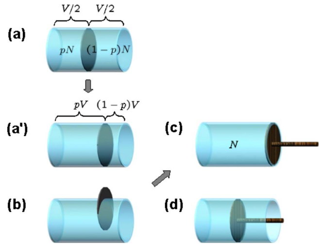
FIG. 4. (Color online) Erasure process for an unbalanced probability distribution. The only difference from the case of balanced distribution (Fig. 3) is the expansion from (a) to (a'), which gives us H(p) bits of work.
