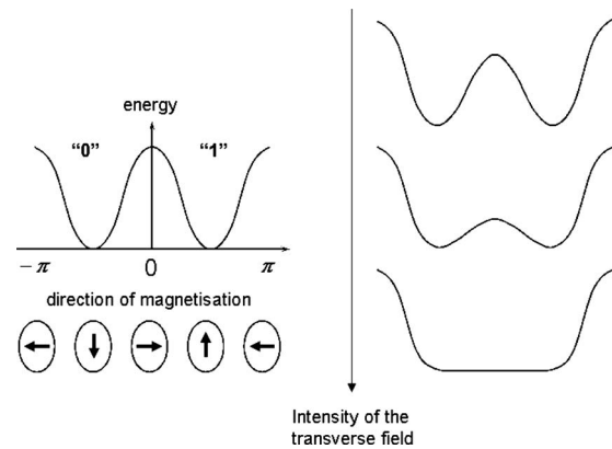
FIG. 2. Potential energy for a binary memory whose state is represented by the direction of the magnetization. When there is no external transverse magnetic field the memory is stable in one of the potential wells, which correspond to "0" and "1" of recorded information. The transverse field lowers the height of the barrier at the center. At a certain point, the profile of the potential becomes bathtublike in shape with a flat bottom, where the direction of the magnetization is sensitive to the longitudinal field component. Adapted from Bennett, 1982.
