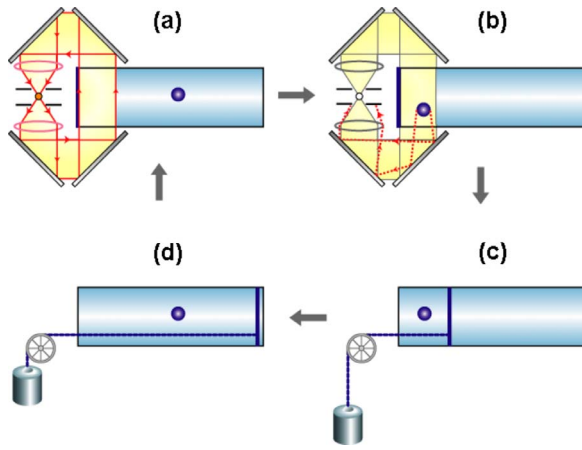
FIG. 5. (Color online) The one-molecule heat engine considered by Gabor to show that the light needs to behave like a wave. When the molecule comes into the illuminated region, a piston is automatically inserted and the “gas” expands isothermally to extract work from the heat bath. This process could in principle be repeated infinitely, converting an infinite amount of heat into mechanical work, if the light had only a particle-like nature. Adapted from Fig. 7 in Gabor, 1961 .
