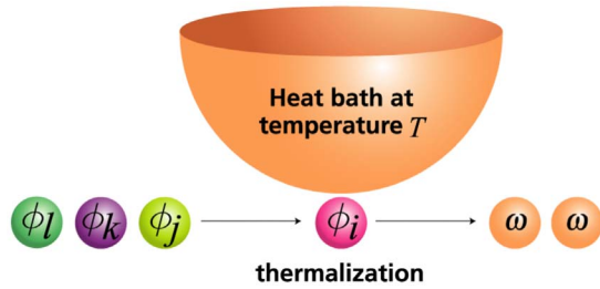
FIG. 10. (Color online) The erasure of classical information carried by quantum states. Each message state interacts with a heat bath at temperature T and reaches thermal equilibrium. The information originally encoded in a state is lost and all states end up in \omega , which is the thermal state at the temperature T .
