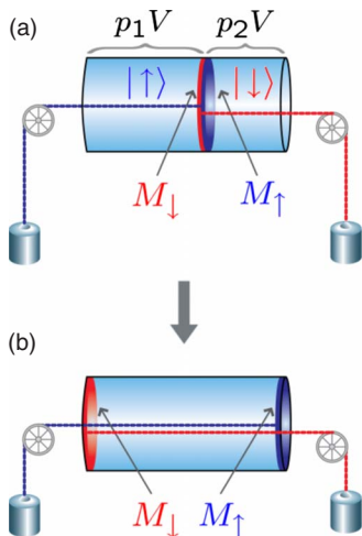
FIG. 7. (Color online) The work-extracting process with semipermeable membranes. In the initial state (a), the vessel is divided into two parts by an impenetrable opaque partition. The left side of the vessel, whose volume is p_1V , is occupied by the |\uparrow\rangle gas, and the right side is filled with |\downarrow\rangle gas. By replacing the partition with two semipermeable membranes M_\uparrow and M_\downarrow we can extract H(p_1) = -p_1 \log p_1 - p_2 \log p_2 bits of work by isothermal expansion. The membranes reach the end of the vessel in the final state (b).
