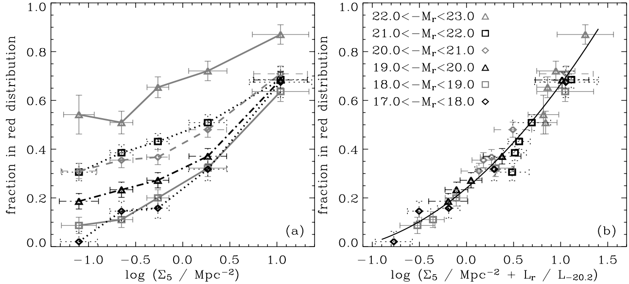
FIGURE 6. The fraction of galaxies in the red distribution as a function of environmental density. Panel (a) uses the projected density \Sigma_5 [same as Fig. 3(a)] while Panel (b) uses a combination of the projected density and the r -band luminosity (normalized by the luminosity for M_r = -20.2 ). (b): The solid line represents a fit to the data points using all luminosity bins.
