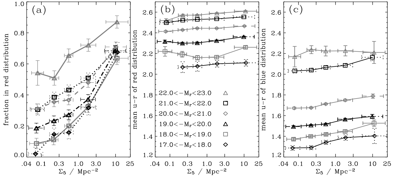
FIGURE 3. The fraction of galaxies in the red distribution (a) and the mean color of each distribution (b, c) as a function of environmental density. The lines and symbols represent different luminosity bins. (b, c): The average change in the mean color over a factor of 100 in \Sigma_5 is 0.05 \pm 0.01 and 0.11 \pm 0.02 for the red and blue distributions, respectively. These shifts were determined using weighted averages from straight-line fits over the six luminosity bins.
