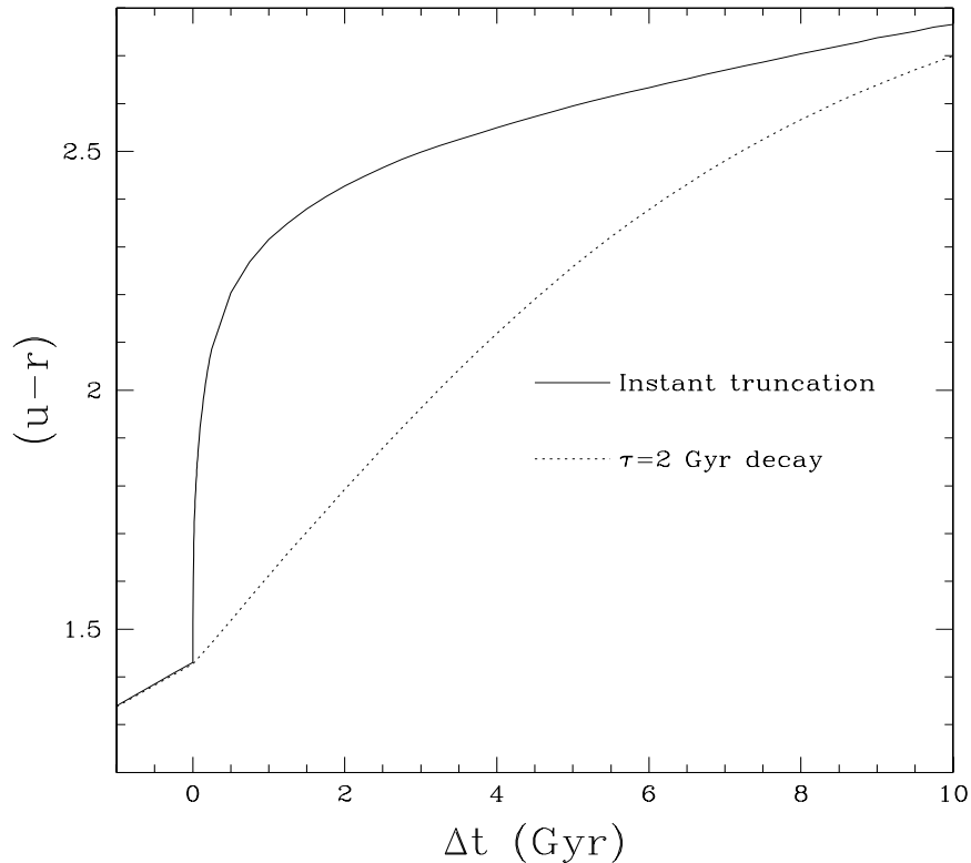
FIGURE 7. The u-r color evolution of two models in which the SFR is reduced at time \Delta t = 0 . Both models are initially evolved for 7 Gyr ( \Delta t < 0 ) using a Salpeter IMF and an exponentially declining SFR with a timescale \tau = 4 Gyr. The solid line represents a model in which star formation completely ceases at \Delta t = 0 , while the dashed line represents a model in which the SFR decreases exponentially with \tau = 2 Gyr.
