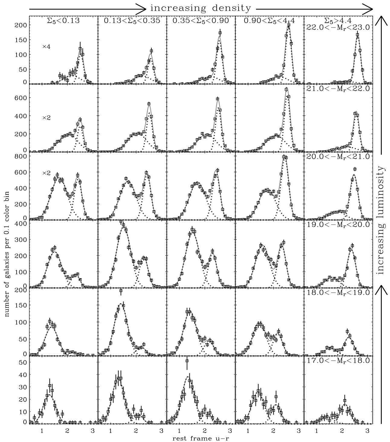
FIGURE 2. Galaxy color functions in bins of environmental density ( \Sigma_5/\text{Mpc}^{-2} ) and luminosity ( M_r ). The squares represent the data points with error bars, while the gray solid lines represent the double-Gaussian fits. The dotted lines represent the individual Gaussian functions. Plots where the counts have been scaled are marked \times 2 or \times 4 .
