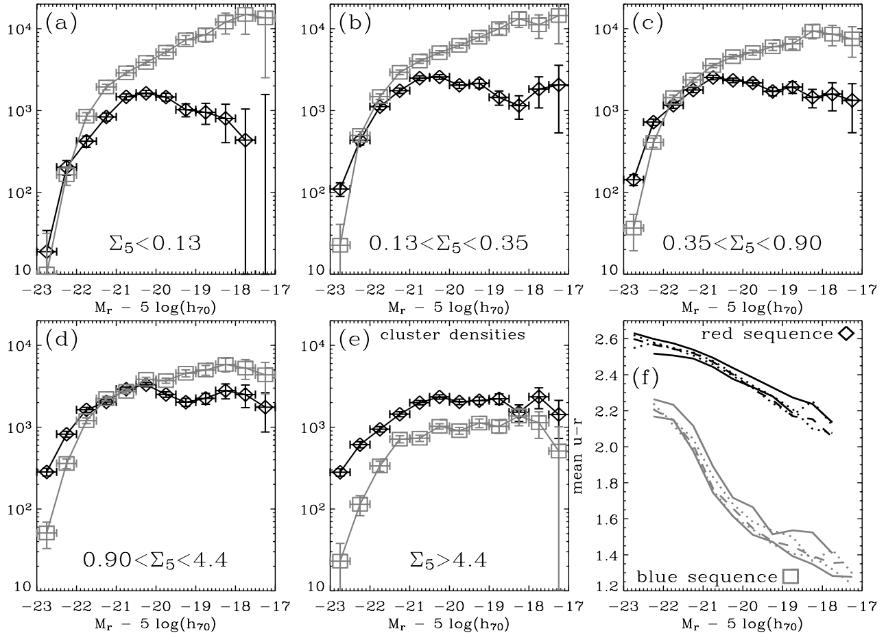
FIGURE 4. (a–e): Luminosity functions for different environmental densities. The gray squares represent the blue sequence while the diamonds represent the red sequence. The y-axis scale represents the completeness-corrected number per magnitude from the 0.01 < z < 0.08 sample ( \sim 10^7 \text{ Mpc}^3 ). (f): Color-magnitude relations for all densities. The solid lines represent the lowest and highest density bins; the dashed line, the middle density bin; and the dotted lines, the remaining bins. The sequences become slightly redder with increasing density (see also Fig. 3); and they are only plotted where the error in the u-r value is less than 0.07 and 0.12 for the red and blue sequences, respectively (typical formal errors are 0.01–0.04).
