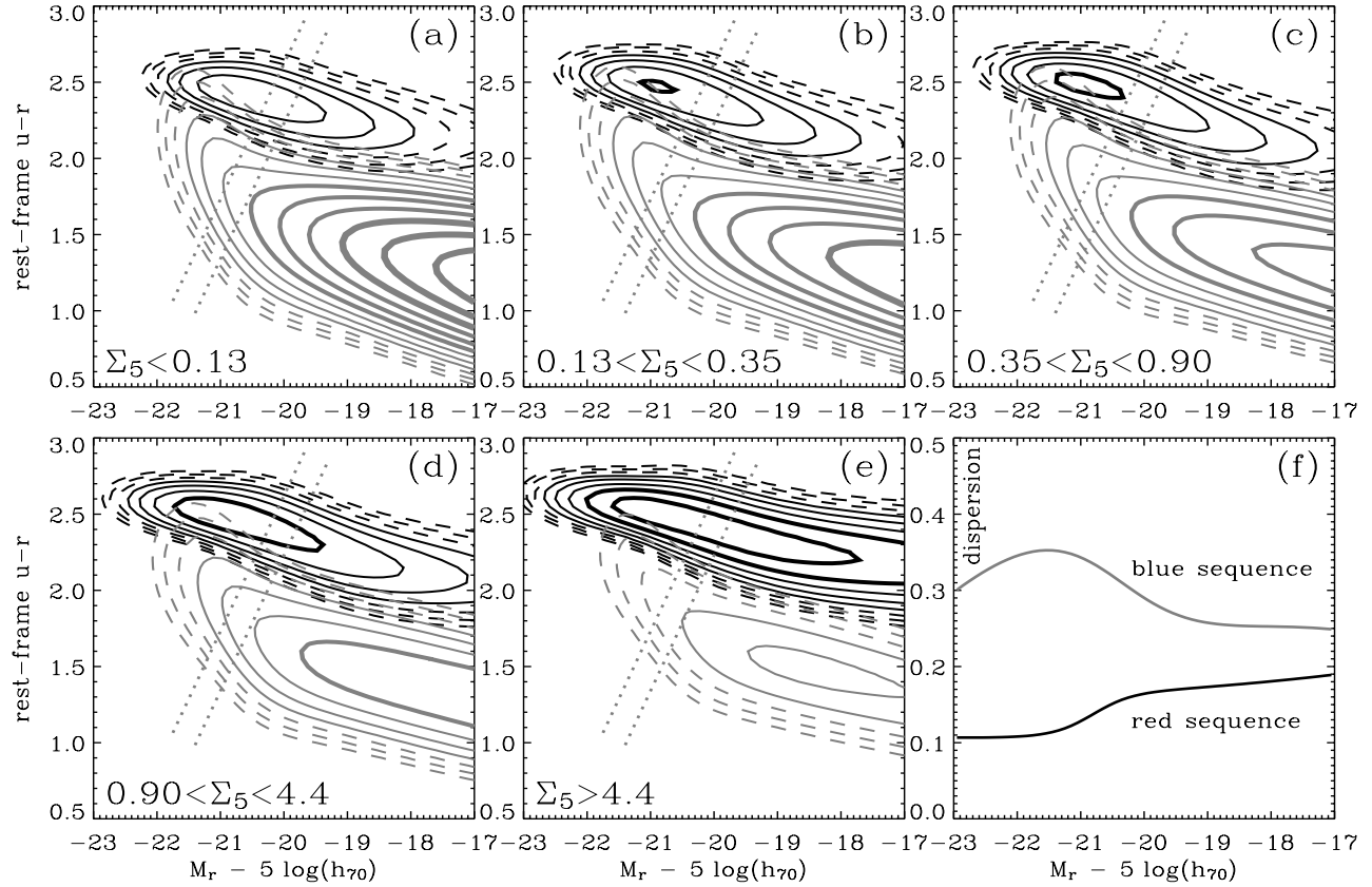
FIGURE 5. (a–e): Parameterized reconstructions of the color-magnitude distributions as a function of environmental density (normalized by total luminosity density). The gray contours represent the blue sequence while the black contours represent the red sequence. For this figure: the fitted means and dispersions have been smoothed using tanh functions plus a straight line or a quadratic; and the luminosity functions using single or double Schechter functions [17]. The dotted lines represent galaxies that have similar stellar masses (see Fig. 1). (f): Dispersion versus magnitude used for each sequence derived from the best fit on the assumption that the dispersion does not vary with density. Note that the measured dispersion includes observational uncertainties. The changes in dispersion are not obvious in Panels (a–e) because changes in the contours are generally dominated by the effects of the luminosity functions.
