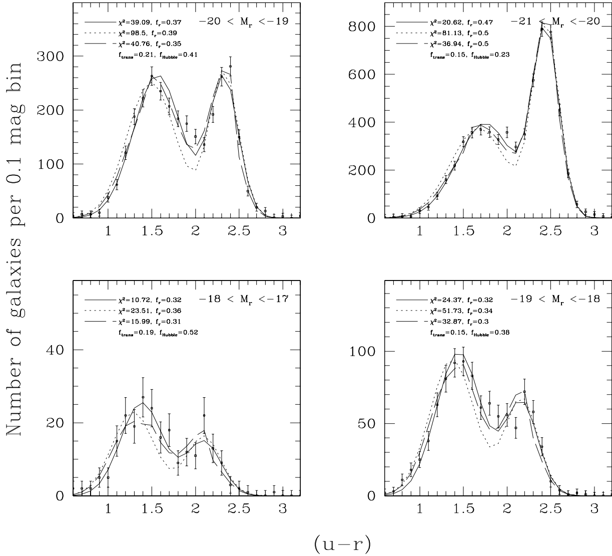
FIGURE 8. Modeling the bimodality. Observed color distributions ( points with error bars ) are shown for four luminosity bins, restricted to the second-highest density bin ( 0.9 < \Sigma_5 < 4.4 ). The solid line shows the double-Gaussian model (Fig. 2), where the mean and amplitude of each Gaussian are fit as free parameters. The dotted line shows the best fit obtained with the mean of the blue distribution constrained to be the same as in the fit to the lowest density bin ( \Sigma_5 < 0.13 ). The dashed line shows the best fit obtained by adding a third component, consisting of a population of galaxies with colors intermediate between the two peaks, with a distribution given by the rate of color evolution in the \tau = 2 Gyr model (Fig. 7). The \chi^2 values and the fraction of galaxies in the red distribution ( f_r ) are shown in the legend for all of these models. For the third model, the fraction of the total galaxy population comprised by these transforming galaxies at the present day ( f_{\text{trans}} ) and the fraction of galaxies that would have passed through this phase in the last 13.7 Gyr ( f_{\text{hubble}} ), assuming the rate of transformation has been uniform, are also shown.
