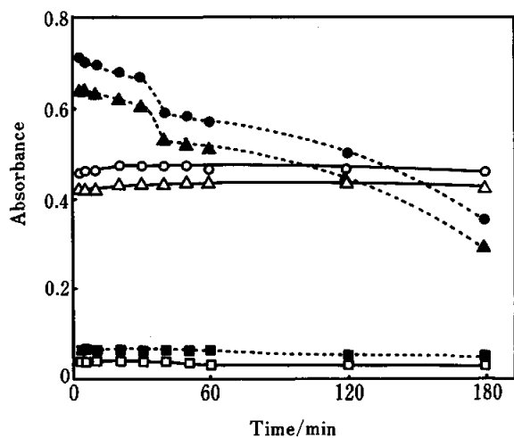
Fig. 3 Effect of PVA on absorbance. \circ , \square and \triangle : with 0.01% (w/v) PVA; \bullet , \blacksquare and \blacktriangle : without PVA; \circ and \bullet : 4 \times 10^{-6} M phosphate; \square and \blacksquare : reagent blank; \triangle and \blacktriangle : ref., reagent blank; molybdate, 0.04 M; \text{H}_2\text{SO}_4 , 0.54 M; Cl-MG, 8 \times 10^{-5} M.
