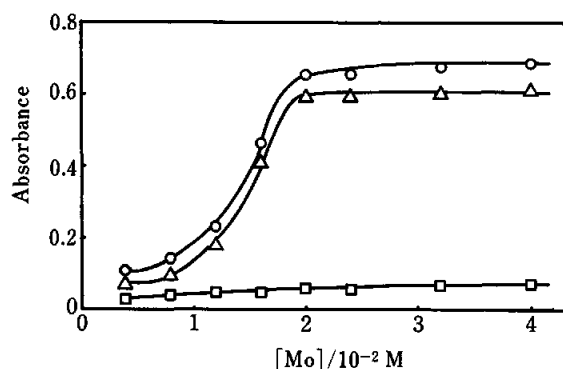
Fig. 5 Effect of the molybdate concentration. \circ : 4 \times 10^{-6} M phosphate; \square : reagent blank; \triangle : ref., reagent blank. \text{H}_2\text{SO}_4 , 0.54 M; Cl-MG, 8 \times 10^{-5} M; PVA, 0.01% (w/v).
