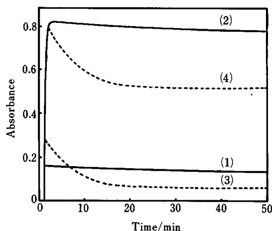
Fig. 2 Absorbance change obtained with MG or with Cl-MG under continuous mixing. (1) and (2): 1 \times 10^{-4} M Cl-MG; (3) and (4): 1 \times 10^{-4} M MG; (1) and (3): reagent blank; (2) and (4): 4 \times 10^{-6} M phosphate. Solution A: 0.08 M molybdate and 0.8 M sulfuric acid with and without 8 \times 10^{-6} M phosphate; solution B: dye solution (pH 5). Solution A and B were mixed rapidly, and absorbances were measured at 650 nm under continuous mixing.
