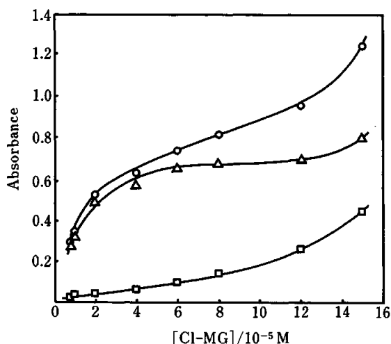
Fig. 6 Effect of the chloro-Malachite Green concentration. ○: 4 \times 10^{-6} M phosphate; □: reagent blank; △: ref., reagent blank. Molybdate, 0.04 M; \text{H}_2\text{SO}_4 , 0.54 M; PVA, 0.01% (w/v).
