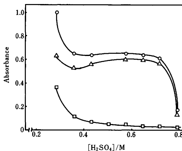
Fig. 4 Effect of the sulfuric acid concentration. \circ : 4 \times 10^{-6} M phosphate; \square : reagent blank; \triangle : ref., reagent blank. Molybdate, 0.04 M; Cl-MG, 8 \times 10^{-5} M; PVA, 0.01% (w/v).
