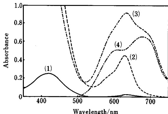
Fig. 1 Absorption spectra of the ion associate of molybdophosphate with Cl-MG. (1) 10^{-5} M Cl-MG (pH 0.3); (2) without phosphate; (3) 4 \times 10^{-6} M phosphate, ref., water; (4) 4 \times 10^{-6} M phosphate, ref., reagent blank. (2), (3) and (4): molybdate, 0.04 M; H 2 SO 4 , 0.54 M; Cl-MG, 8 \times 10^{-5} M.
