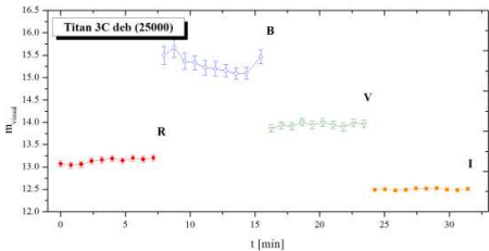
Figure 3. The magnitudes of the Titan 3C R/B debris for B, V, R, I filter (y axis) as a function of time (x axis) obtained during single telescope observations.
