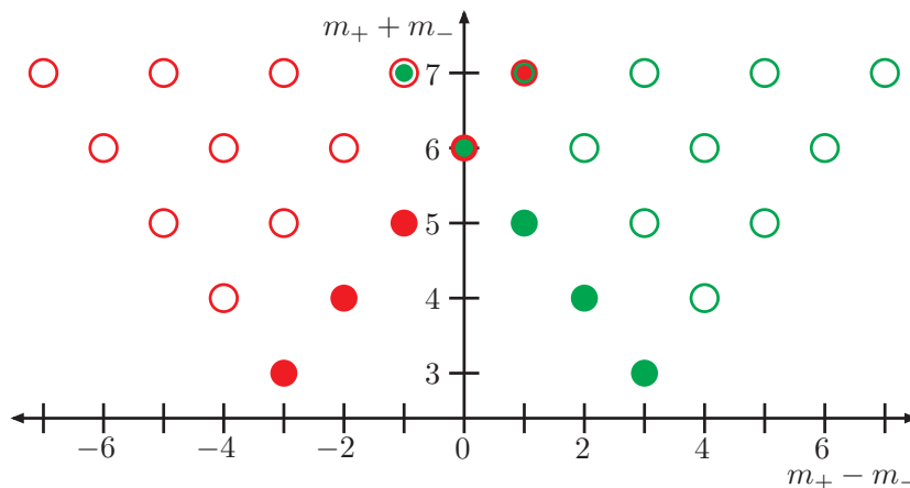
Figure 2. The m -gluon amplitudes produced by the operator F^3 , where m_+ and m_- are the numbers of positive- and negative-helicity gluons, respectively. The left tower (red circles) of amplitudes is the self-dual sector, produced by F_{SD}^3 . The right tower (green circles) is produced by the anti-self-dual operator F_{ASD}^3 . For MHV ( \overline{\text{MHV}} ) amplitudes with exactly three negative (positive) helicities, the circles are filled. The figure is from ref. [29].
