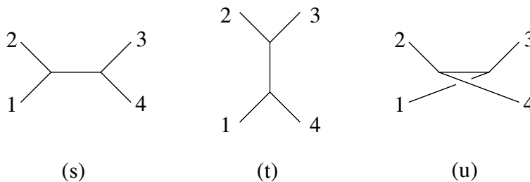
Figure 1. The three cubic graphs at the four-point level.
