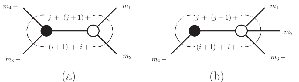
Figure 3. Next-to-MHV F^3 amplitudes are constructed by sewing together two MHV vertices, one for F^3 (white circle) and one for ordinary gauge theory (black dot). There are two distinct ways of distributing the four negative-helicity gluons, (a) and (b). The dotted lines indicate that an arbitrary number of positive-helicity gluons may be present.
