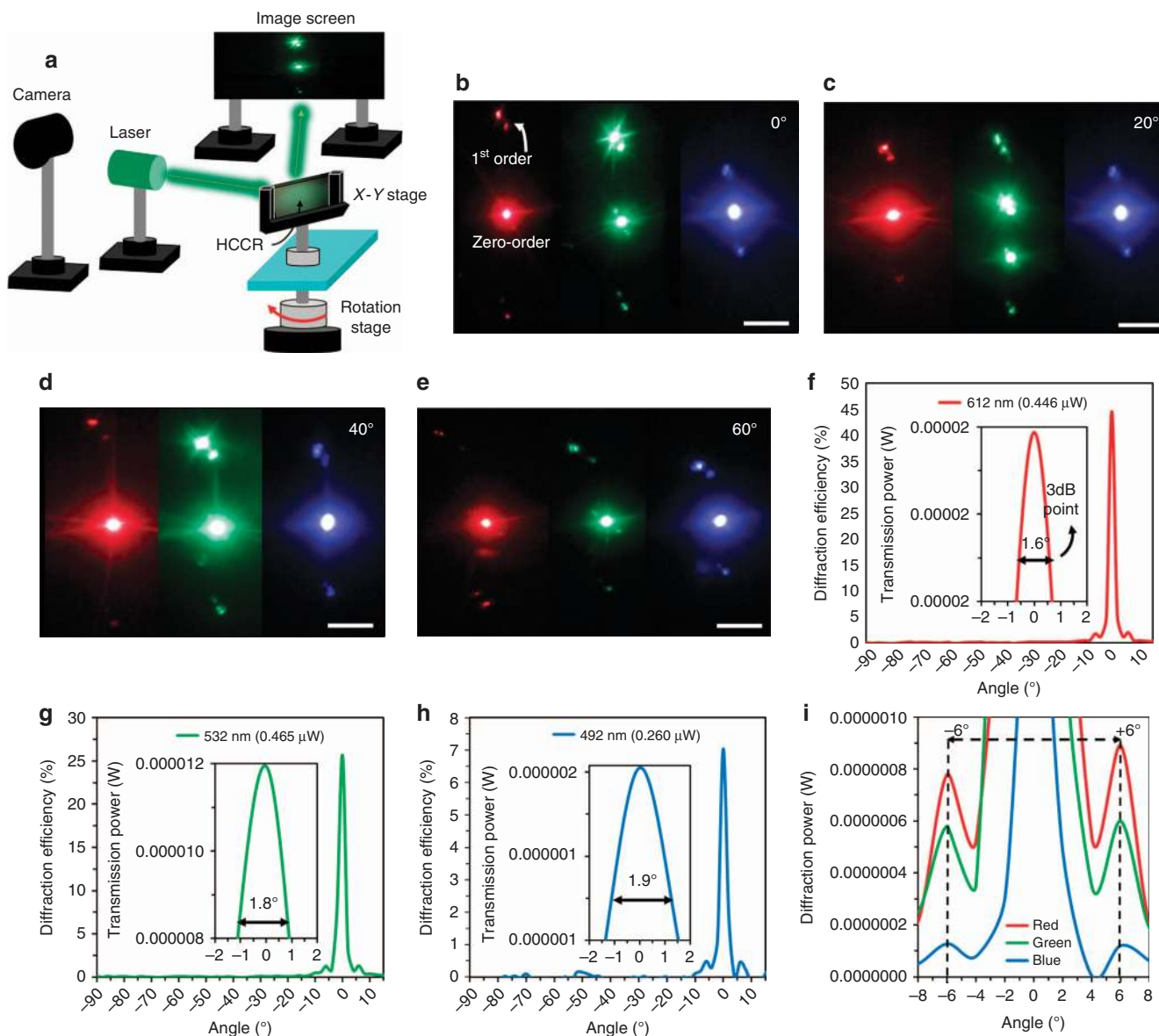
Figure 4 Characterization of visible diffraction from the HCCR array. (a) Experimental setup used for shining laser light on the HCCR array at various angles and projecting the diffracted light on a screen. (b–e) The diffraction patterns in response to red, green and blue laser light, irradiated at incidence angles from 0° to 60°. Scale bars = 2 cm. (f–i) Angular DE measurement of the HCCR. The DE and intensity in response to red, green and blue laser light at rotation angles from –90° to +90°. The DE and intensity decrease as wavelength increases; however, the angular spread of the non-diffracted spot at the 3 dB point increases.
