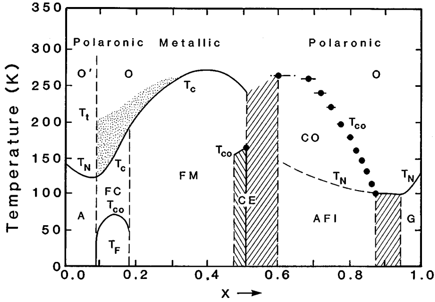
Fig. 1. Phase diagram for the system \text{La}_{1-x}\text{Ca}_x\text{MnO}_3 for O' -orthorhombic/ O -orthorhombic c/a < \sqrt{2} , c/a > \sqrt{2} . Here T_t = O'-O transition temperature, T_{co} = charge and orbital ordering temperature, \bullet = T_{co} for n/(n+2) with integral n and 2 \leq n \leq 14 , T_N = Néel temperature and T_c = Curie temperature. Further, CO = charge and orbital ordering; A,G = canted-spin Type-A, Type-G antiferromagnetic insulator; CE = Type-CE antiferromagnetic insulator; FC, FM = ferromagnetic conductor, metal; T_F = tetragonal, charge-ordered ferromagnetic insulator. The speckled area is the region of CMR.
