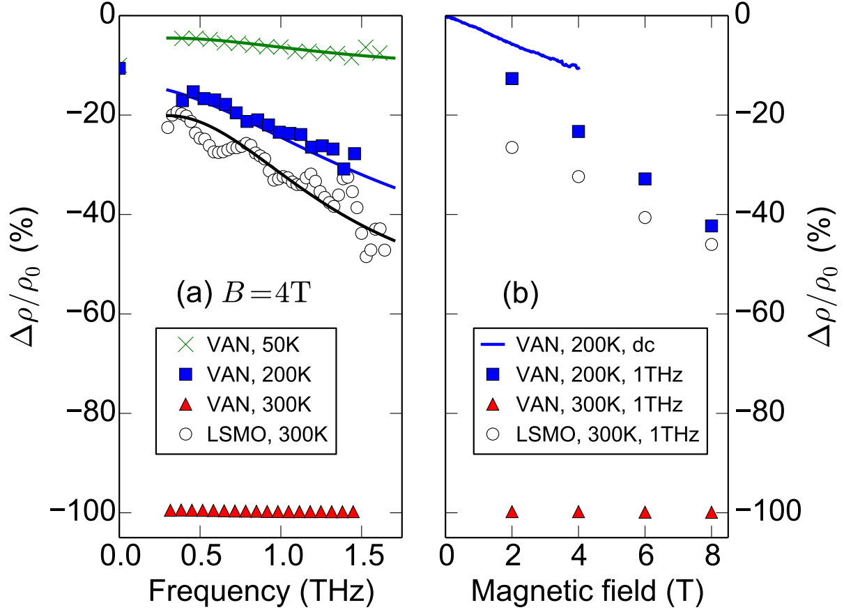
Figure 4: (a) Frequency-dependence of the colossal THz MR of the LSMO-ZnO VAN at B = 4\text{ T} for T = 50\text{ K} (green crosses), T = 200\text{ K} (blue squares) and T = 300\text{ K} (red triangles). Data for the pure LSMO film at T = 300\text{ K} are also shown (circles). Fits with the Drude-Lorentz model are given by the solid lines. (b) Magnetic-field dependence of CMR. Data obtained from dc magnetotransport (solid line) on the VAN at T = 200\text{ K} can be compared with the MR at 1.0 THz (blue squares). At 300 K and 1.0 THz, the THz MR approaches 100 % for the VAN (red triangles), while it is smaller for the pure LSMO film (circles).
