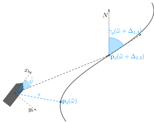
FIGURE 6. Illustration of key concepts for navigation with respect to path following. The path reference point p_d(\bar{\omega}) , i.e. point yielding the closest Euclidean distance to the vessel, is here located right of the vessel, while the look-ahead reference point p_d(\bar{\omega} + \Delta_{LA}) is located a distance \Delta_{LA} further along the path.
