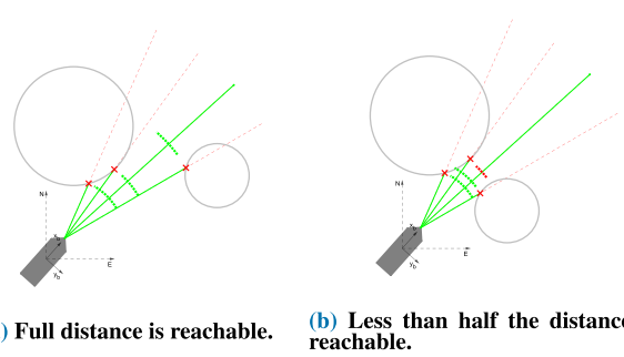
FIGURE 10. Illustration of the feasibility algorithm for two different scenarios. After sorting the sensor indices according to the corresponding distance measurements, the algorithm iterates over them in ascending order, and, at each step, decides if the vessel can feasibly continue past this point. In the scenario displayed in the figure on the right, the opening is deemed too narrow for the full distance to be reachable.
