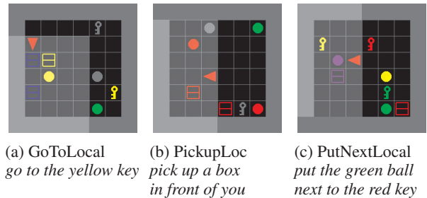
Figure 1: Instructions and initial states for three BabyAI tasks. In (b), a memory in a reward model is necessary to determine success which depends on the initial position.
