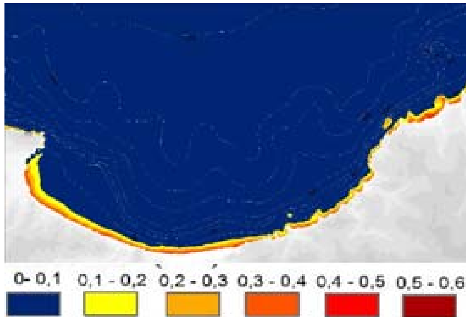
Fig. 7: Maps of the current orbital speed
