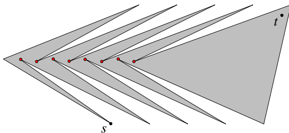
Figure 1: \lfloor \frac{n}{2} \rfloor - 1 beacons are sometimes necessary to route between a pair of points in a simple polygon. Here, n = 19 and 8 beacons are required to route from s to t .
