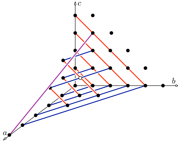
FIGURE 1. The M -subgraphs of \mathbb{N}^3 for Example 5.4.
