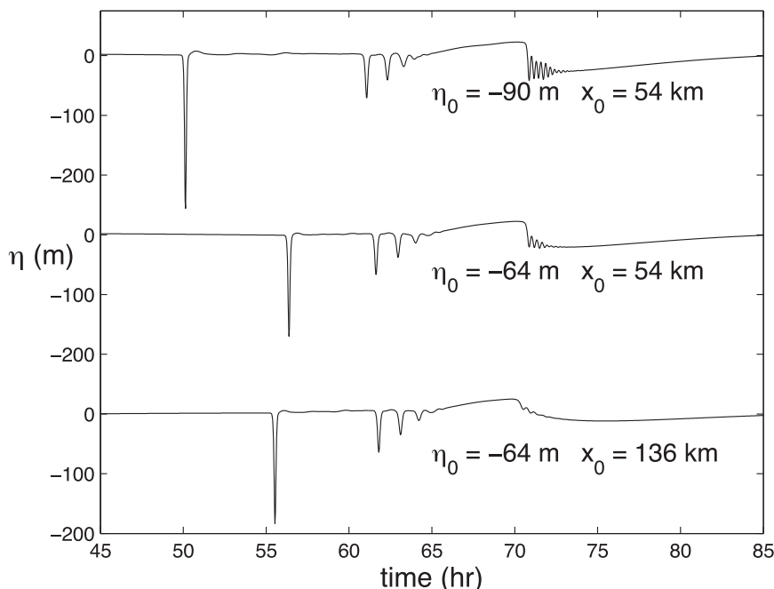
FIG. 6. Time series of Ostrovsky equation (12) solutions for the northern topography at x = 380 km for a solitary wave with amplitude \eta_0 and initial location x_0 as indicated.
