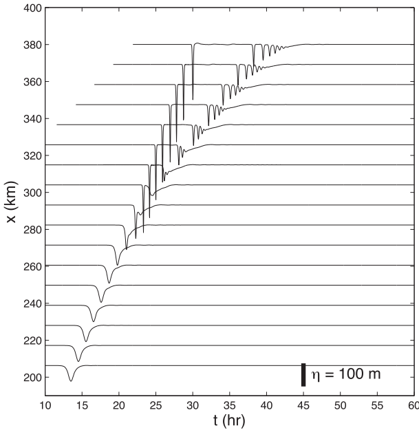
FIG. 4. Numerical solution of the variable coefficient Ostrovsky equation (12) for the northern topography with no rotational effects ( \gamma = 0 ). The initial wave has amplitude \eta_0 = -64 m at x_0 = 54 km. Time series of wave amplitude \eta(x, t) at selected x locations on the slope are shown. The scale on the lower right indicates wave amplitude.
