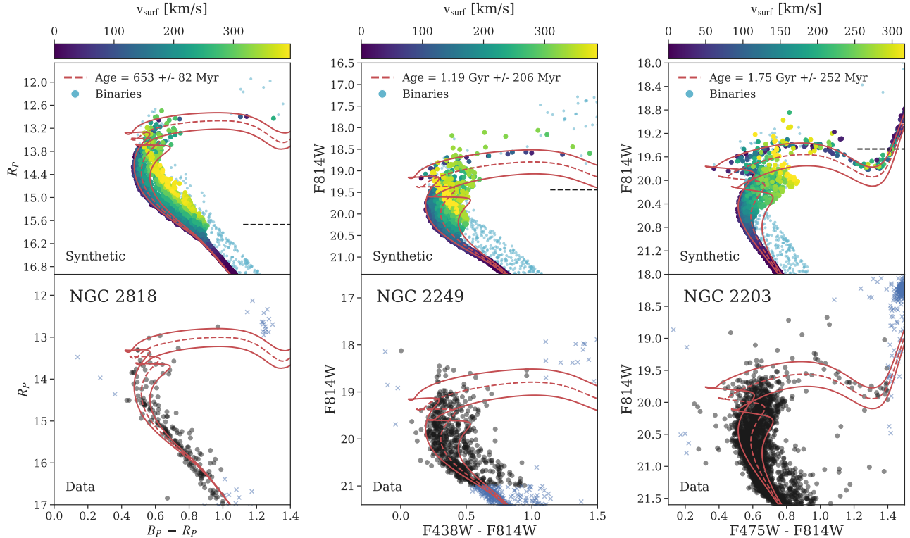
FIG. 2.— Top row: synthetic clusters, with each point color coded by the stellar model’s average surface velocity. These points were generated at a single age of 0.7, 1, and 1.5 Gyr, from left to right. Binaries are shown as cyan points. Solid red lines mark the youngest and oldest age non-rotating MIST isochrones that span the eMSTO width; rotation effects can mimic this span. The red dashed lines show the mean age. Turn off masses (left to right): 1.5 - 1.8 M_{\odot} , 1.60 - 2.15 M_{\odot} , 2.1 - 2.85 M_{\odot} , respectively, according to our models. The black dashed line approximately marks the magnitude below which our velocities are ramped down as a proxy for magnetic braking. Bottom row: data for NGC 2818, 2249, and 2203 as black dots, with the same non-rotating isochrones from above overlaid for comparison. Blue crosses are data excluded from the fits.
