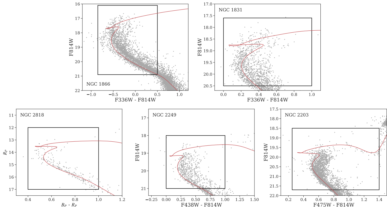
FIG. 1.— CMDs of our five chosen star clusters, in order of descending age: NGC 1866, 1831, 2818, 2249, 2203. Black rectangles show the CMD area used for fitting models to data. Red (non-rotating, MIST) isochrones represent SSPs according to our adopted cluster parameters, listed in the text. The red clump is ignored in our fits, for reasons explained in the text.
