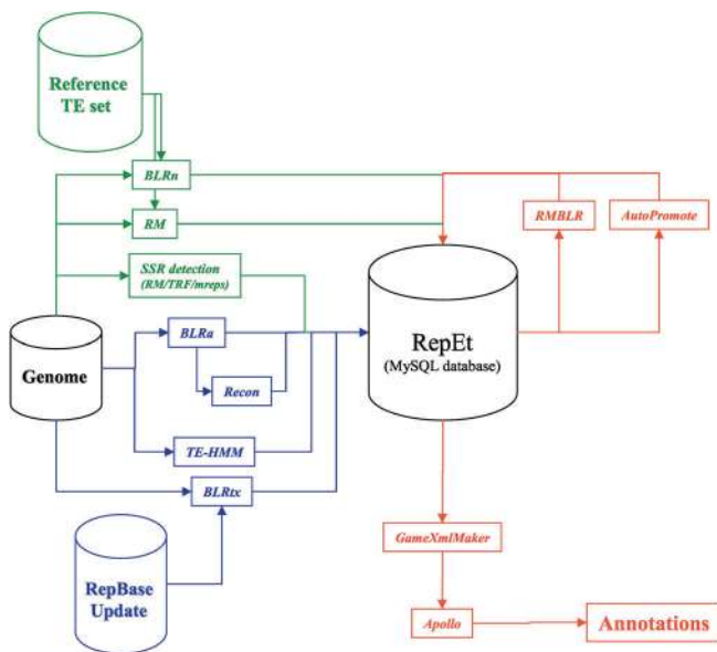
Figure 1. Schematic of Our TE Annotation Pipeline
