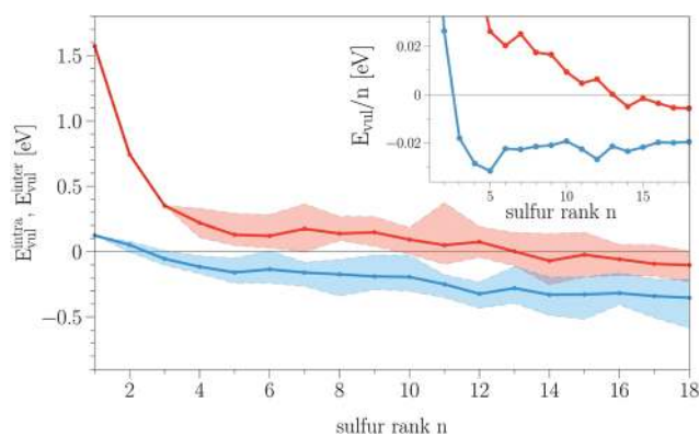
Fig. 6 The vulcanization energies E_{vul}^{intra} (eqn (5)) for intra-chain reactions (red) and E_{vul}^{inter} (eqn (6)) for inter-chain reactions (blue). The colored areas represent the results of all sampled conformations, and the solid lines show the averaged trends. In the inset, the vulcanization energies normalized by the sulfur rank E_{vul}/n are shown.
