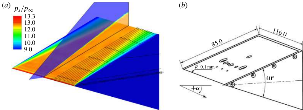
FIGURE 5. (Colour online) Surface pressure normalized by the free-stream static pressure on the wedge probe at \text{AoA} = 0^\circ and Mach 7.4 in HEG, left. Basic probe dimensions, right. All dimensions are provided in millimetre.
