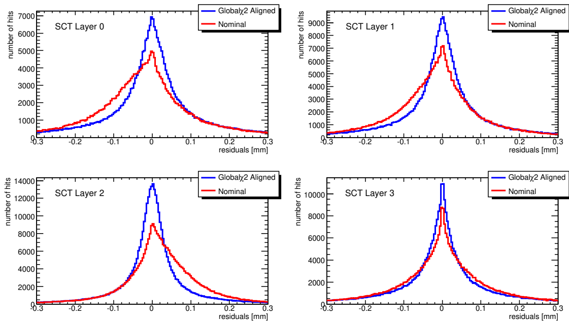
Figure 32. The SCT biased residuals for the different layers of the SCT are shown before (red) and after (blue) the alignment.
