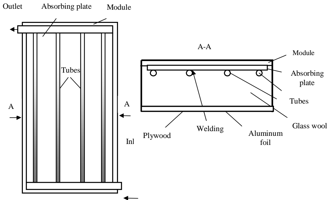
Fig. 2: Design of PVT Collector.
