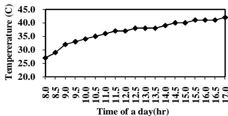
Fig. 4: The temperature of water in the tank vs day time for a variable cloudy day.
