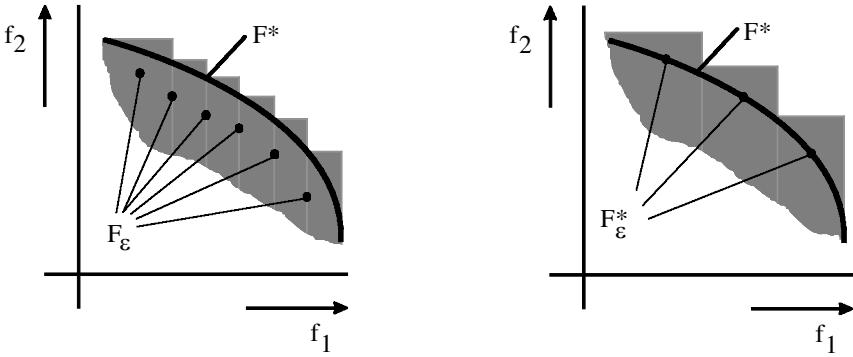
Figure 3: Graphs visualizing the concepts of t -approximate Pareto set (left) and t -Pareto set (right).
