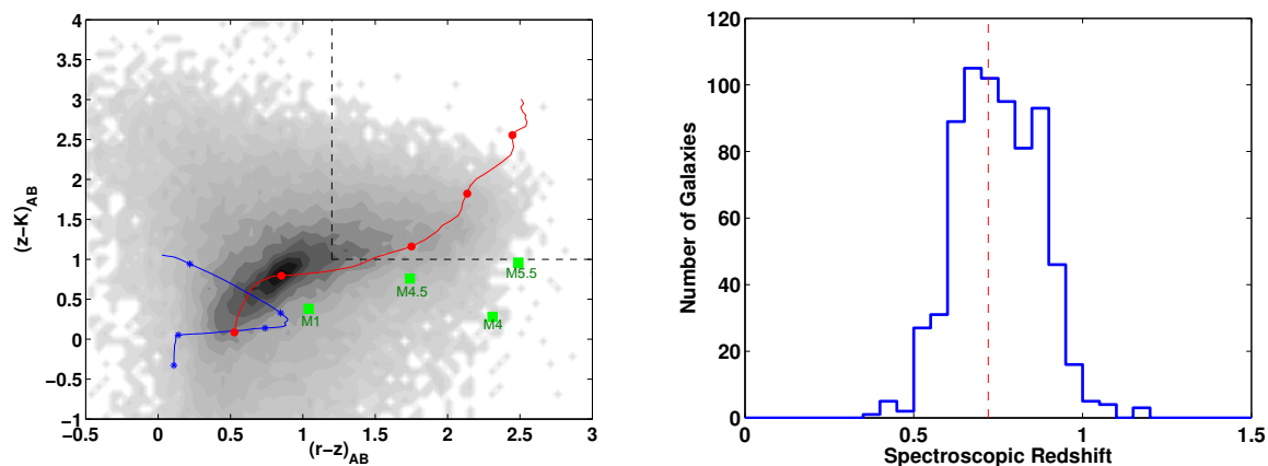
Figure 11. Left: Source density plot showing galaxies in the SN-X3 field in the DES+VISTA (r-z) versus (z-K) colour-colour plane. The red line represents the colour of a typical early-type galaxy template from Jouvel et al. (2009) in the redshift range 0 < z < 2 while the blue line shows a late-type galaxy template from the same work. The green squares denote some representative colours of early-type M-stars from Leggett et al. (2000), which have very similar optical colours to LRGs but are significantly bluer in terms of their infrared colour. Markers indicate redshift steps of 0.4 in these tracks. Our high-redshift LRG selection box for OzDES is represented by the top right of the plot. Right: Redshift distribution of all LRG targets in the field that have secure redshift identifications. The median redshift of 0.72 is marked with a vertical line.
