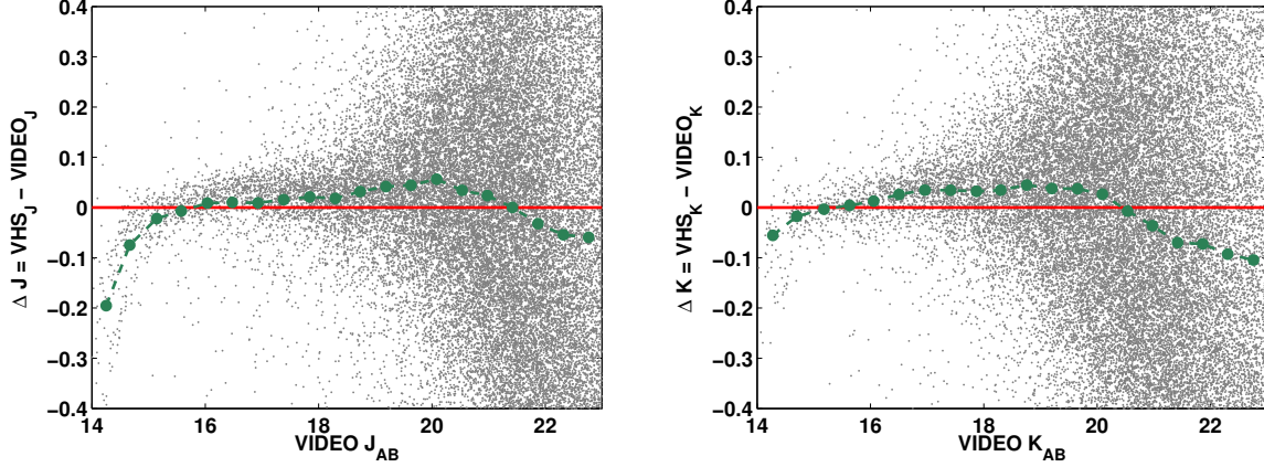
Figure 5. Difference between the SEExtractor VHS forced photometry magnitudes and deeper VISTA VIDEO catalogue magnitudes in the J and K_s bands as a function of the VIDEO near infrared magnitude. The dashed line corresponds to the median trend whereas the solid line marks an offset of 0 mag. The median offsets are +0.04 mag in J and +0.03 mag in K_s relative to VIDEO at the bright end where the logarithmic magnitude distributions are expected to be roughly Gaussian.
