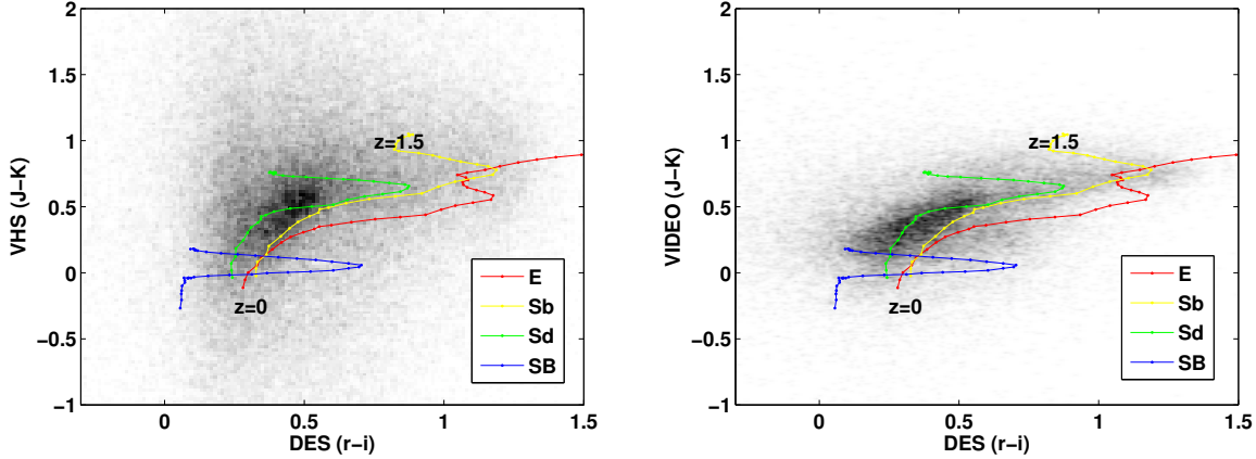
Figure 7. The grey clouds show source densities of galaxies in the DES+VISTA (r-i) versus (J-K) colour-colour plane for both our DES+VHS forced photometry catalogue (left) and DES+VIDEO catalogue (right). The coloured tracks mark the expected colours of galaxies from Jovel et al. (2009) for four different galaxy templates spanning the full range of galaxy types in those catalogues. The tracks go from redshift 0 to 1.5 with points marking redshift intervals of 0.04. The observed colours of our galaxies in the DES+VISTA catalogue, overlap well with the predicted colours of galaxies from Jovel et al. (2009) but the larger spread in the (J-K) colours in VHS relative to VIDEO results from the larger photometric scatter on the shallower VHS data.
