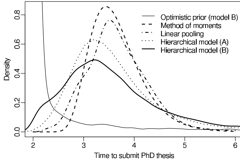
Figure 5: Marginal elicited prior predictive densities of X based on: pooled (mixture model) (---), plug-in (-), hierarchical approaches, method A (· · ·) and method B (thick solid line) and prior predictive density (thin solid line).
