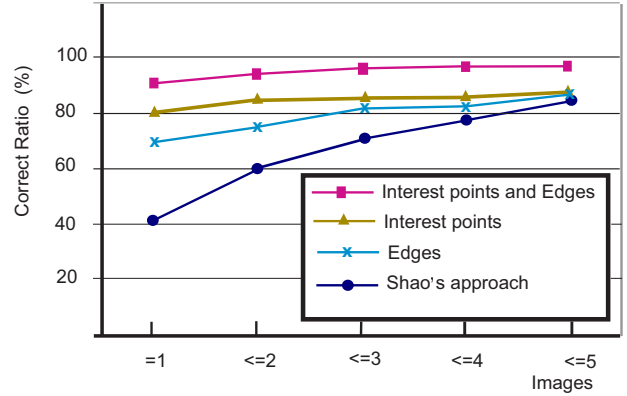
Fig. 2. Comparison of the correct ratio of our system with that of Shao [10]. Experiments are conducted on the ZuBuD image database. y (Vertical axis) is the correct ratio. The correct retrieval result is ranked within the top x (Horizontal axis) of the retrieved views.
