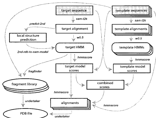
Fig. 2. The SAM-T02 prediction process consists of several parts: building a multiple alignment for the target sequence using the SAM script target2k , predicting secondary structure with predict-2nd , building HMMs for the target sequence with the SAM script w0.5 , scoring the template library against the target HMMs using the SAM program hmmscore , scoring the target sequence against the template HMMs with hmmscore , combining scores to select templates, choosing target-template alignments, generating fragments with the SAM program FRAGFINDER , and doing fragment packing with UNDERTAKER .
