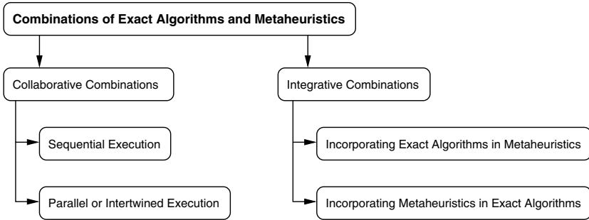
Fig. 1. Major classification of exact/metaheuristic combinations
