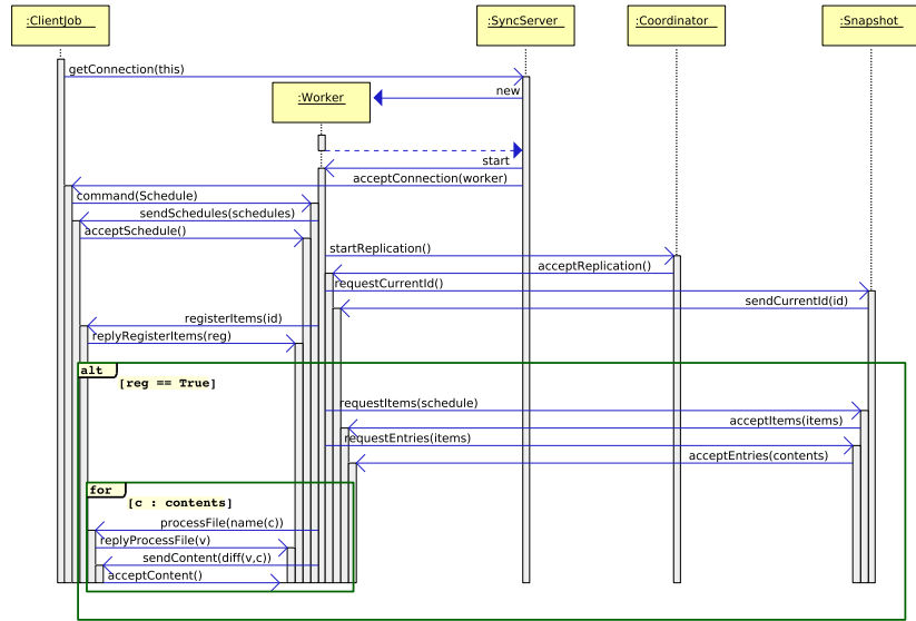
Figure 6.4: Replication interaction
