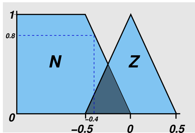
Figure 4.3: Fuzzifications for conditional features
