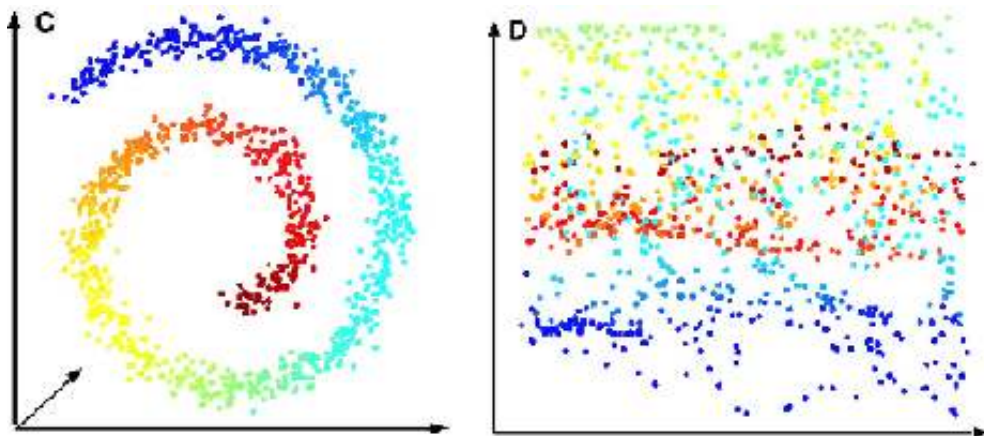
Figure 2.8: The “Swiss roll” dataset with zero-mean normally distributed noise and the resulting Isomap embedding ( \varepsilon = 5 ) [8]
