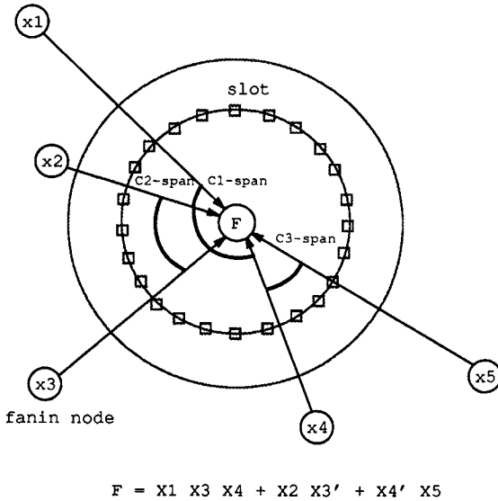
FIGURE 3 Cube ordering viewed as a linear assignment problem.
