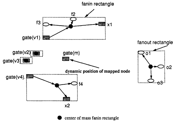
FIGURE 5 Dynamic updating of placement positions (Euclidean norm).
