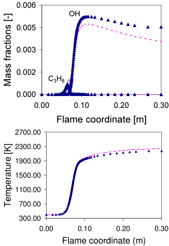
Figure 2.1: Intermediate species (OH and C 3 H 8 ) and temperature profile ( \Delta = Williams, - = Curran).
