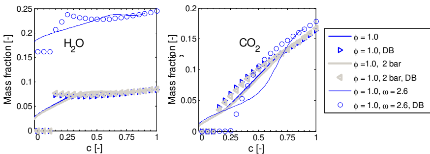
Figure 3.5: Effect of steam dilution and pressure on (left) H 2 O and (right) CO 2 in PREMIX solutions (solid lines) and database solutions (symbols)
