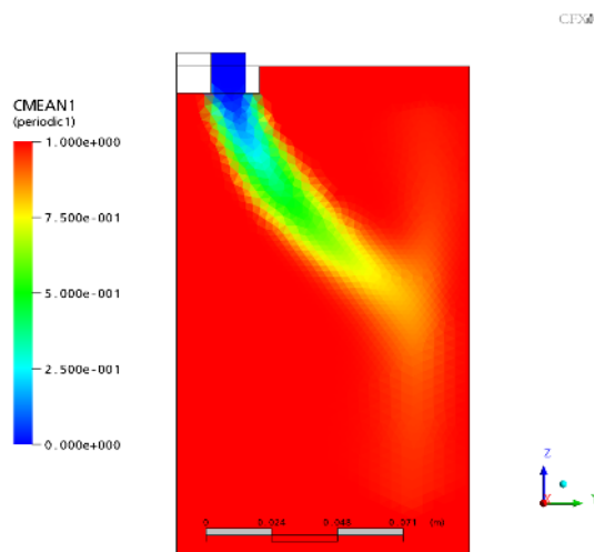
Figure 5.3: The predicted field of the reaction progress variable.
