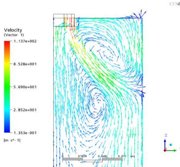
Figure 5.2: Vector plot of the predicted velocity field.
