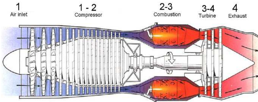
Figure 1.2: A cross sectional view of a gas turbine engine (courtesy of Rolls Royce)
