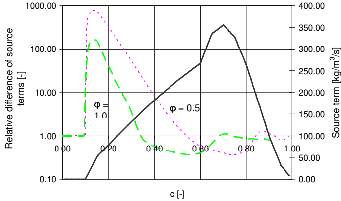
Figure 4.6: Laminar database comparison of c source term with PREMIX solution for \phi = 0.5 and \phi = 1.0 (solid = database source term at \phi = 0.5 , dashed - \frac{S_{c,Database}}{S_{c,PREMIX}} for \phi = 1.0 )
