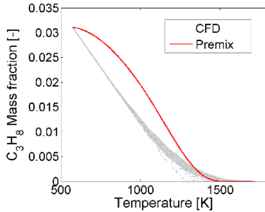
Figure C.2: The concentration of C_3H_8
