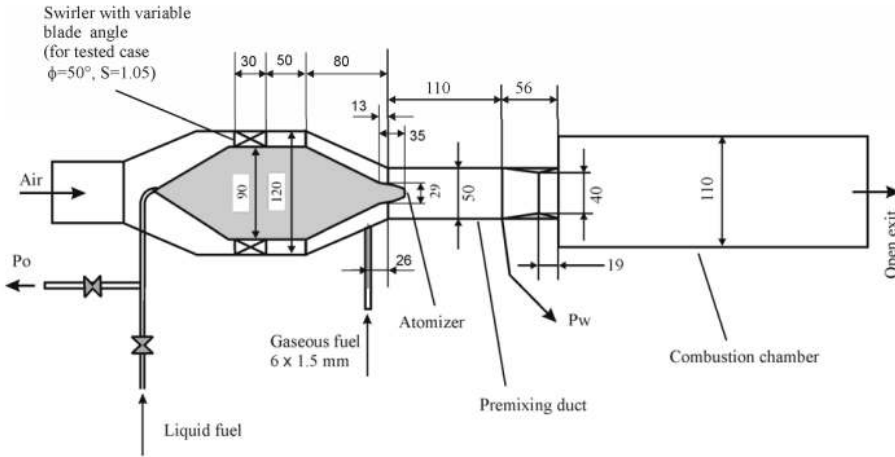
Figure 4.8: Experimental setup
