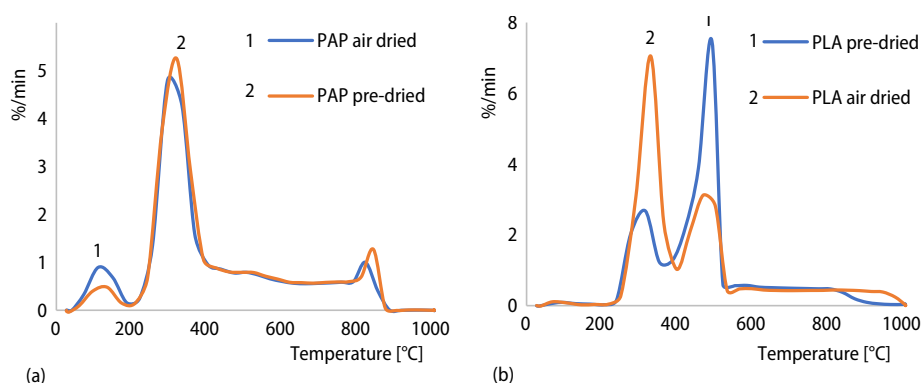
Figure 1. The DTG curves of the air dried paper (a) and plastic (b) raw materials compared to their respective pre-dried samples
