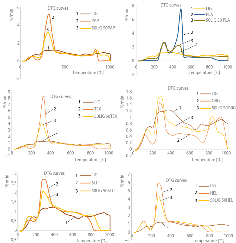
Figure 3. Comparative DTG curves of the samples of paper, plastic, textile, organics, sewage sludge, sunflower shells and their blends with 50 wt.% lignite
