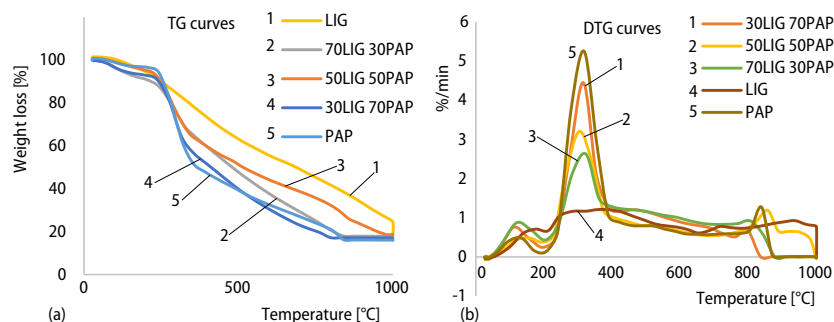
Figure 2. The TG (a) and DTG (b) curves of the samples of lignite, paper and their blends in proportions of 30, 50, and 70 wt.%
