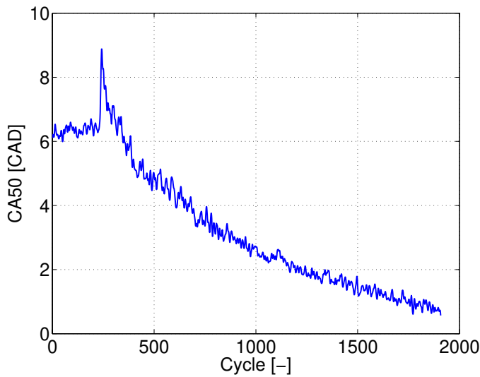
Figure 4: CA50 (CAD ATDC) corresponding to Figure 3.
