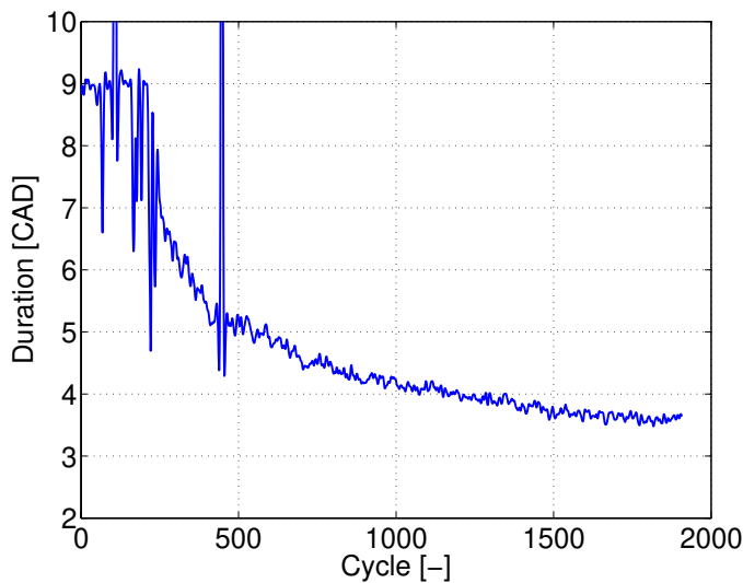
Figure 5: Combustion duration corresponding to Figure 3.
