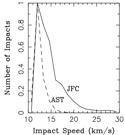
Figure 14. Model distributions of Earth-impact speed of JFC (solid line) and asteroidal (dashed) particles with D = 200 \mu\text{m} . Since the effects of the gravitational focusing have been accounted for in the calculation, the minimum impact speed is equal to the escape velocity from Earth's surface, or about 11.2 \text{ km s}^{-1} . The majority of JFC particles have impact speeds in the 11.2\text{--}15 \text{ km s}^{-1} range. JFC particles with larger impact speeds have lower impact probability but are important for interpretation of the meteor radar data (e.g., Wiegert et al. 2009).
