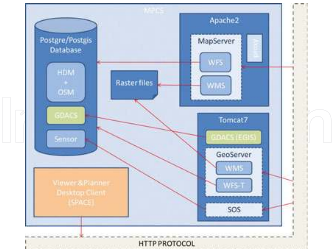
Figure 20. GIS software components (source: ICARUS).
