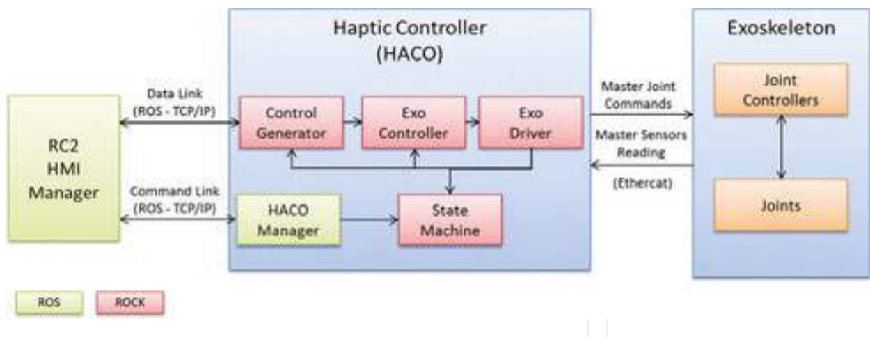
Figure 26. Global software architecture of the exoskeleton device (source: ICARUS).
