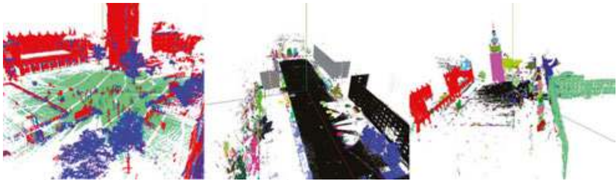
Figure 36. (i) Point cloud classification of data from geodetic scanner. (ii and iii) Scene segmentation examples (source: ICARUS).
