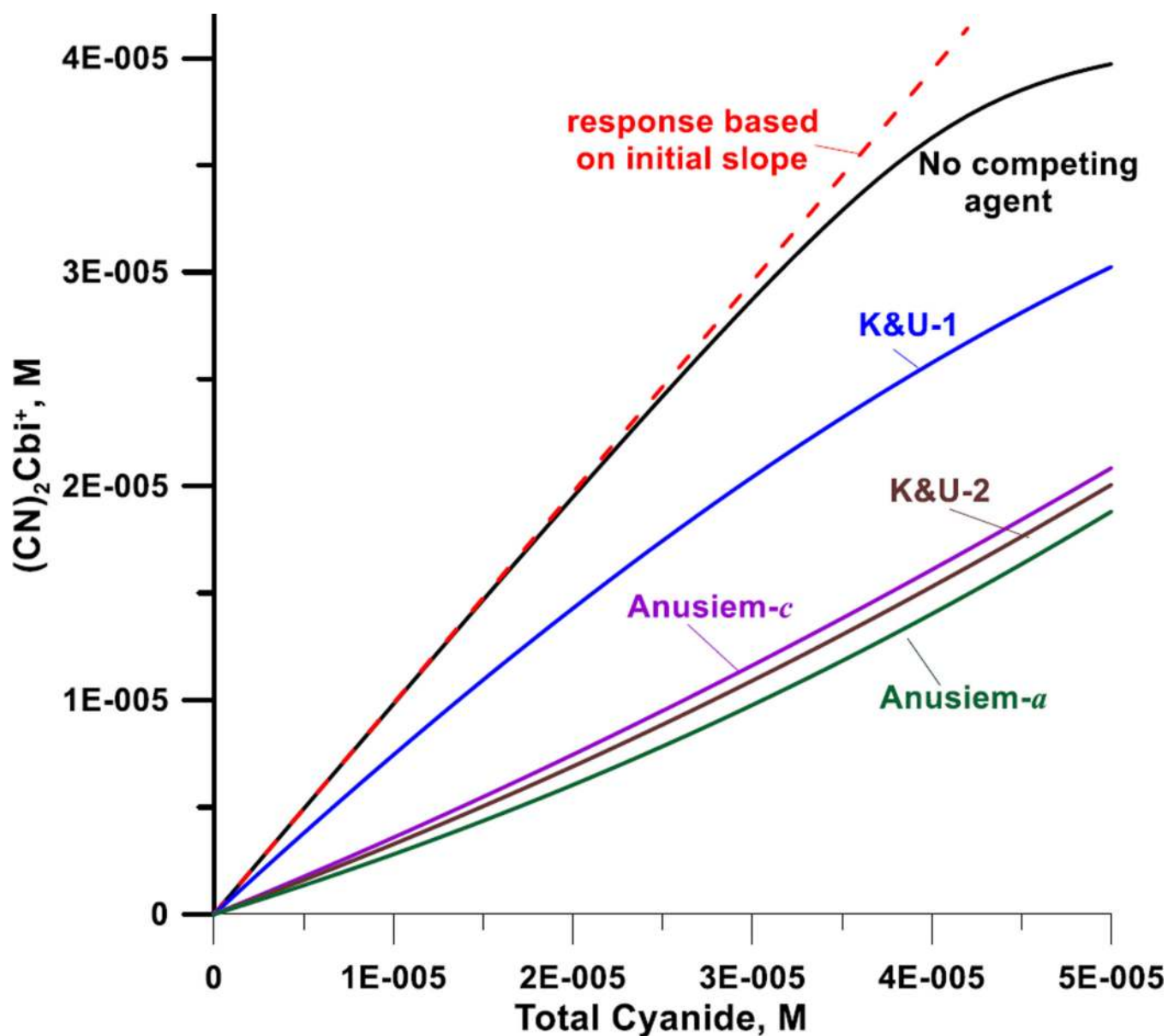
Figure 2. Computed equilibrium 1-CN concentrations vs. total cyanide concentration initially present, 42 \mu\text{M} total 1 added. Solid black line: in the absence of competing agent; Dashed red line: hypothetical case where the initial linear slope observed at very low added cyanide levels is maintained throughout. Other traces represent computations that take into account competition of methHb present (45 \mu\text{M} ) using different sets of methHb-CN binding constants from Klapper and Uchida 31 (K&U-1 and K&U-2) and by Anusiem et al. 32 for methHbA and methHbC (Anusiem-a and Anusiem-c). The computations are based on thermodynamic data, i.e., infinite reaction time is presumed.
