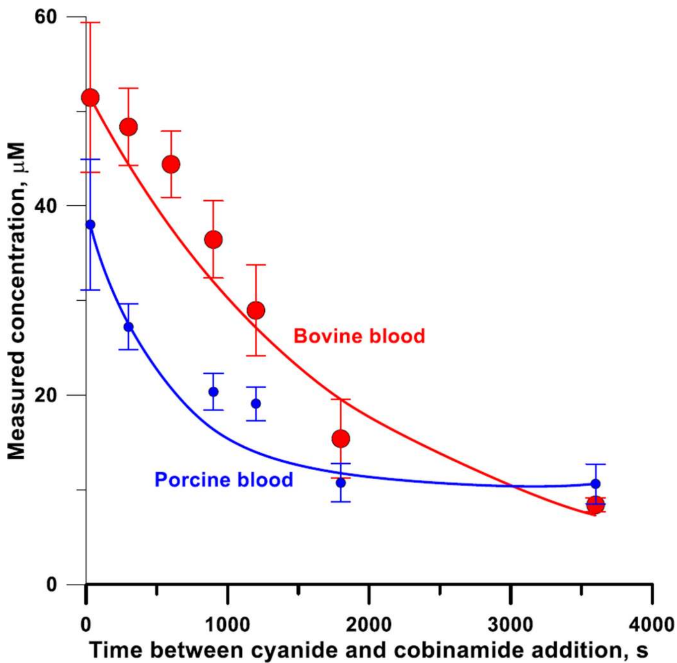
Figure 3. Measured concentration of (CN)_2Cbi vs. the incubation time of CN^- in Bovine and Porcine blood.
