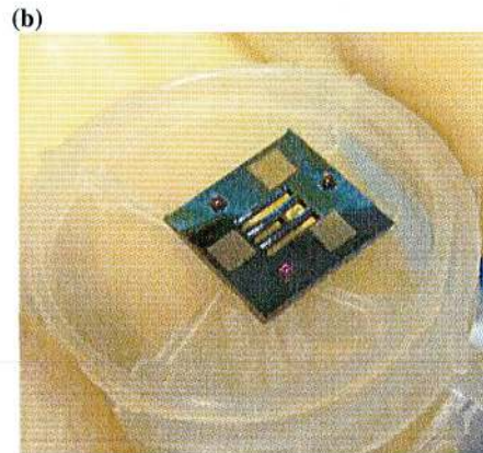
Figure 5. (a) a single zoneplate-array chip mounted onto a removable zoneplate holder. Both the chips and the holder rely on kinematic mounts for accurate, repeatable positioning. (b) The zoneplate array chip is 11-mm wide and contains four free-standing membranes.
