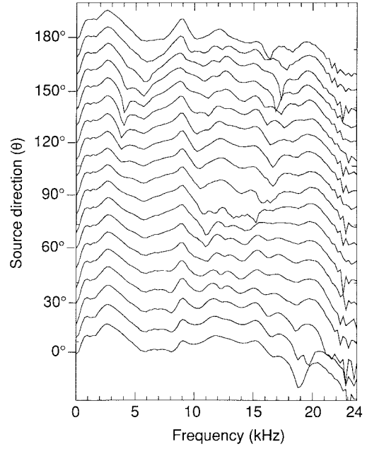
Fig. 3. Frequency responses of the measured HRTF's of the left ear.
