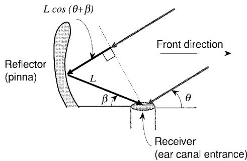
Fig. 9. Simple ear model in which sound is reflected by the pinna.
