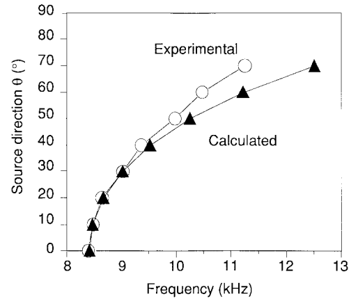
Fig. 10. Frequency variation of nonminimum-phase zero depending on source direction. Circles indicate the zeros extracted using common-acoustical-pole and zero modeling of HRTF's. Triangles indicate the zeros calculated using the simple reflection model.
