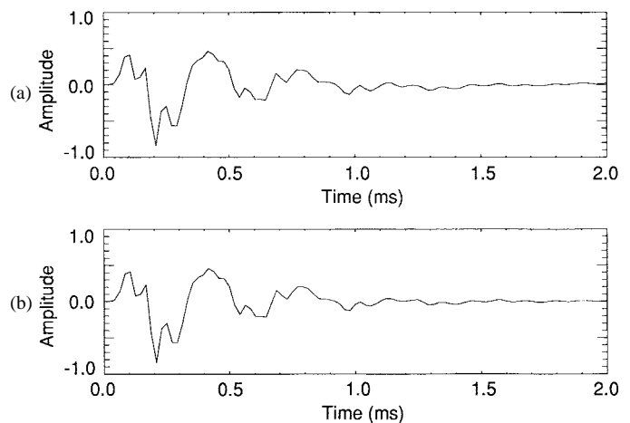
Fig. 6. Impulse responses at 20° of (a) actual HRTF and (b) common-acoustical-pole and zero modeled HRTF.
