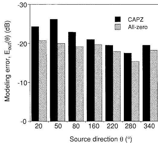
Fig. 5. Modeling errors of common-acoustical-pole and zero model (20 common AR coefficients + 40 variable MA coefficients, black bars) and the conventional all-zero model (60 MA coefficients, gray bars) for HRTF's.
