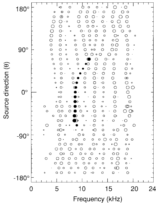
Fig. 7. Zeros for various sound directions. Open circles indicate minimum-phase zeros, and filled circles indicate nonminimum-phase zeros. Circle size corresponds to the distance between the zero and the unit circle on the z -plane (the bigger the circle, the smaller the distance).
