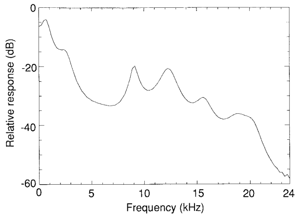
Fig. 4. Frequency response of transfer function with the estimated common AR coefficients.
