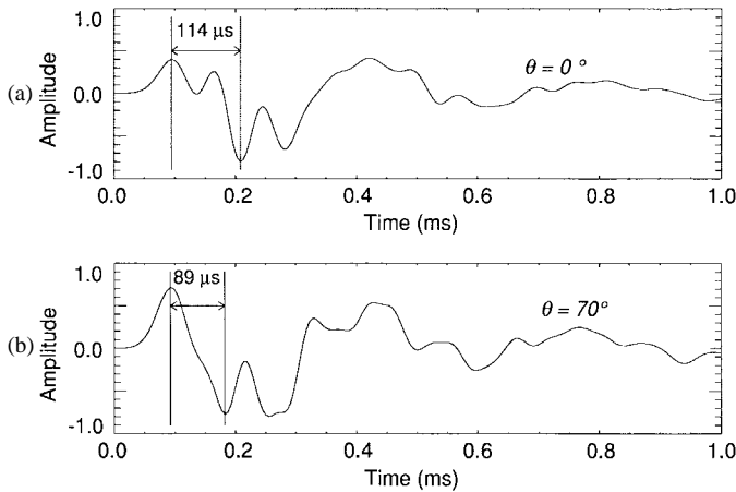
Fig. 8. Impulse responses of (a) 0^\circ and (b) 70^\circ HRTF's. The delay between the direct and reflected sounds decreases as the source-direction angle increases.
