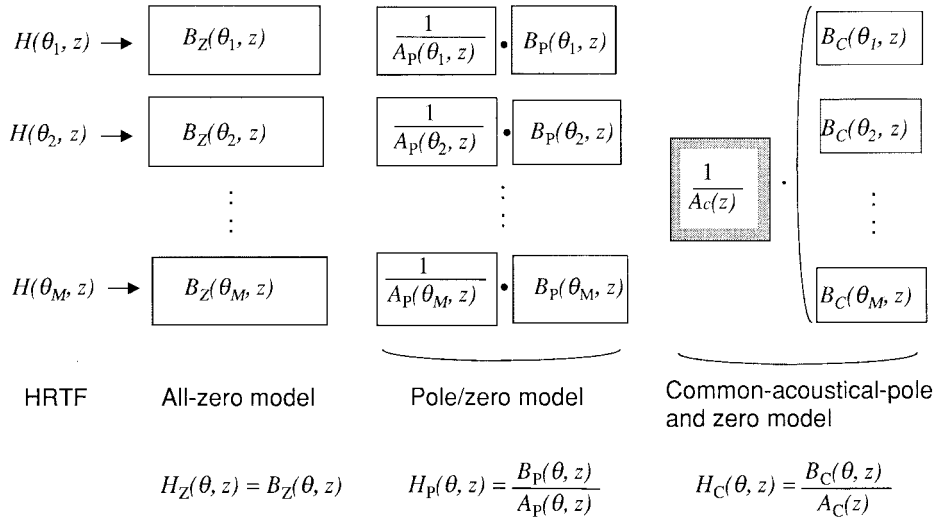
Fig. 2. Modeling of multiple HRTF's corresponding to different source directions, \theta_1, \theta_2, \dots, \theta_M , using an all-zero model, a pole/zero model, and the proposed common-acoustical-pole and zero model.
