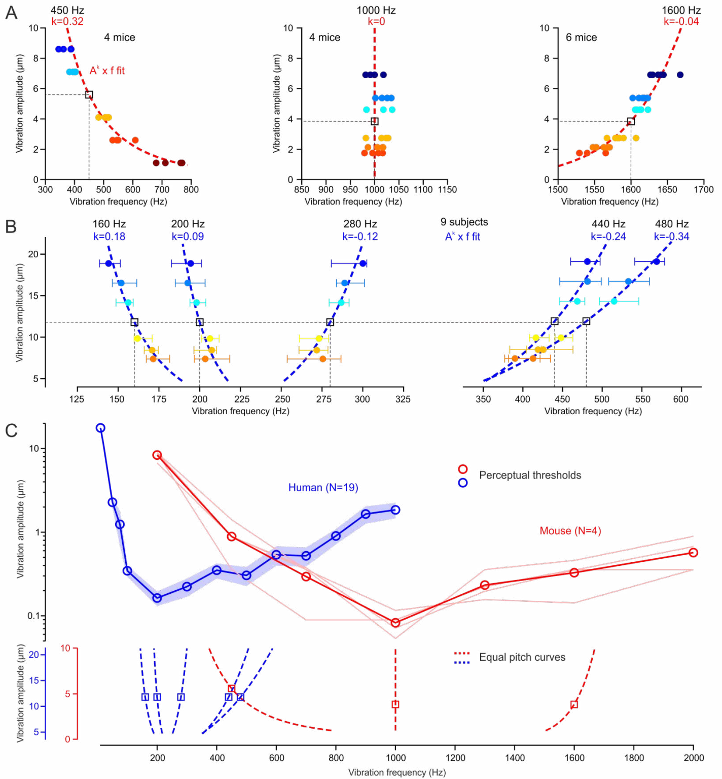
Figure 2. Equal pitch curves slope towards the frequency of maximal vibrotactile sensitivity. A: A^k \times f equal pitch curve fits (red lines) to vibration amplitude as a function of the frequency shift ratio (normalized to the center frequency, black square, see Methods for details) for 450Hz (N=4 mice), 1000 Hz (N=4 mice) and 1600 Hz (N=6 mice) center frequencies (colored symbols). B: A^k \times f equal pitch curve fits (blue lines) to vibration amplitude as a function of the median ( \pm quartiles, colored symbols) frequency shift ratio (normalized to the reference frequency, black square, see Methods for details) of n=9 subjects, for 160 Hz, 200 Hz, 280 Hz, 440 Hz and 480 Hz reference frequencies. C: V-shaped perceptual sensitivity curves (amplitude thresholds as a function of vibration frequency) for mouse (shaded lines: individual mice, symbols: mean) and human (mean \pm s.e.m.). The equal pitch curves for all tested center/reference frequencies are replotted in the bottom panel illustrating that vibratory pitch perception shifts, with increases in amplitude, toward the frequency of highest vibrotactile sensitivity in both mouse (red) and human (blue).
