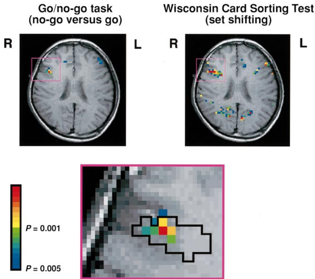
Fig. 5 Spatial overlap of the no-go dominant area with the shift-related area revealed by group analysis. The activity observed 5 s after the no-go trials and 7 s after dimensional changes in the WCST is shown on the left and right, respectively. The no-go dominant area in the right inferior frontal sulcus is enlarged and superimposed on a black frame that encloses the shift-related area.
